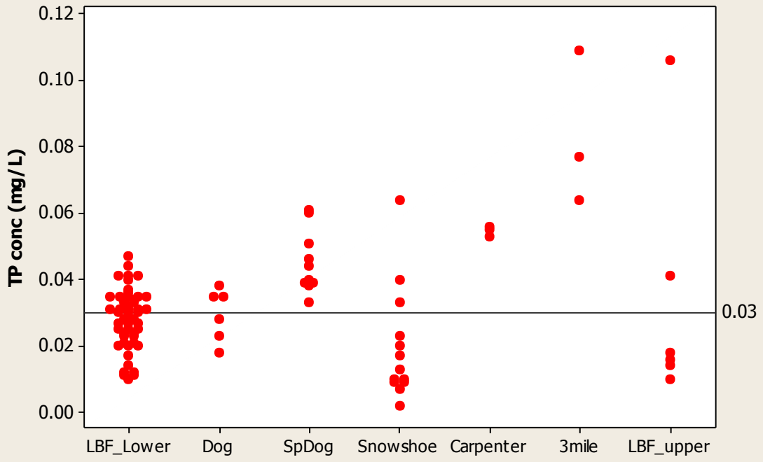
Summer TP Concentrations 1998-2009
