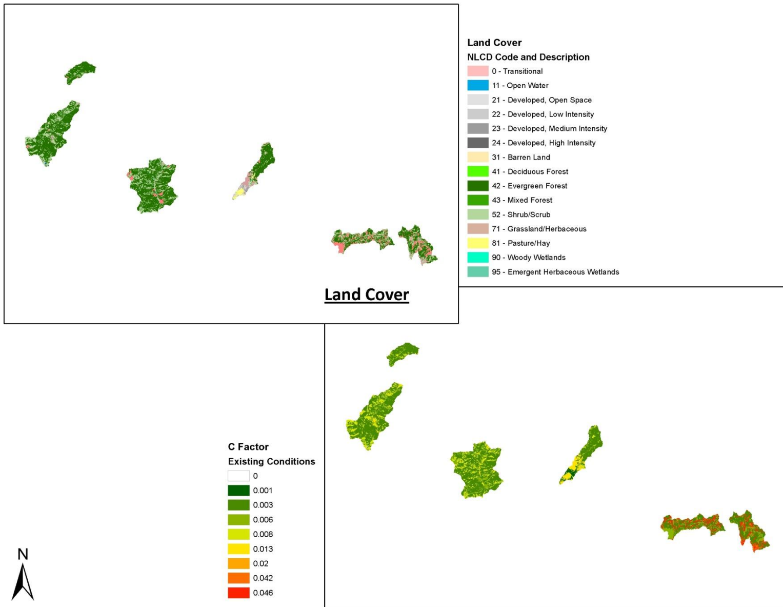
Figure 2-3. Land Cover and C-Factors for the Central Clark Fork Tributaries Project Area
