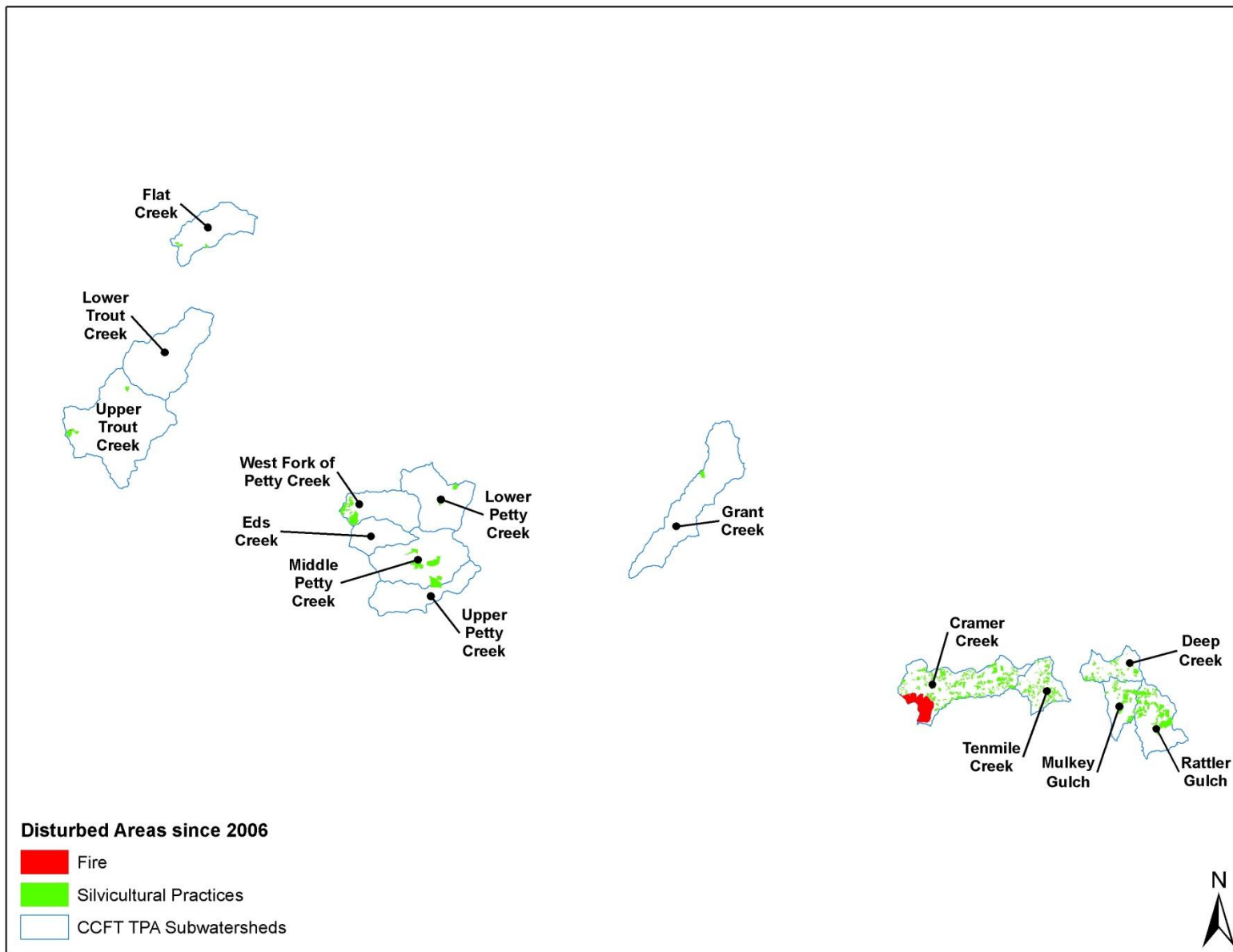
Figure 2-4. Fire and Timber Harvest Areas in the Central Clark Fork Tributaries Project Area since 2006
