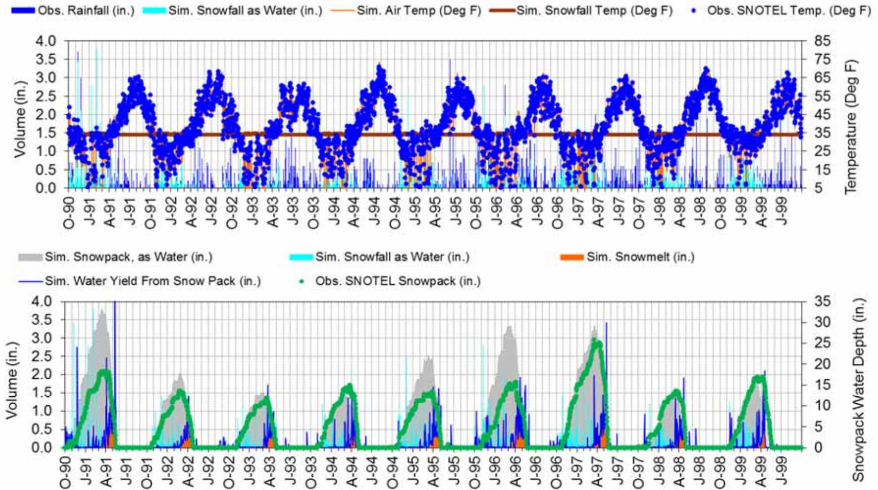
Figure F-12. LSPC snow calibration at GRAVE CREEK (North - 4300ft) (10/1/1990 - 9/30/1999).
