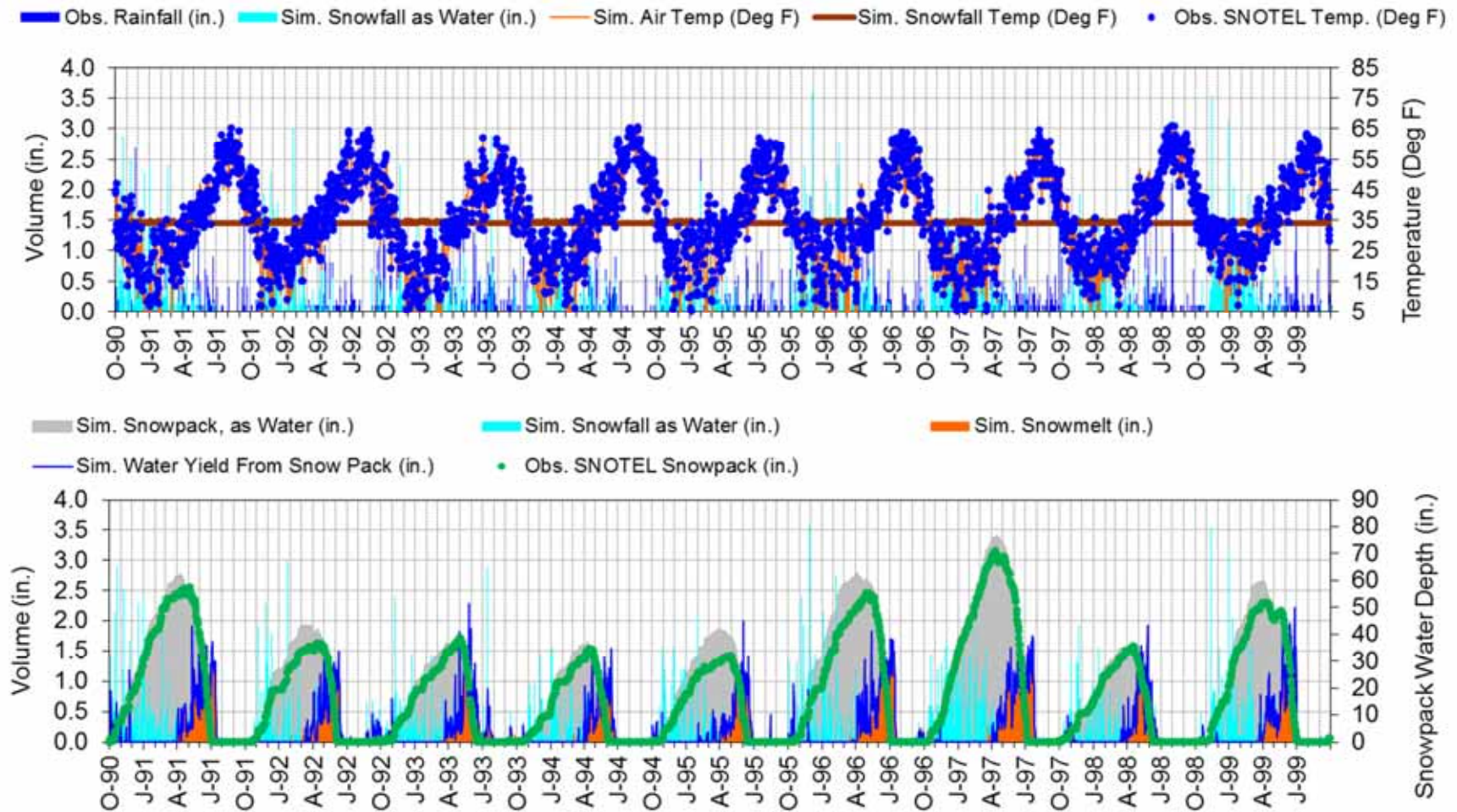
Figure F-26. LSPC snow calibration at NORTH FORK JOCKO (South - 6330ft) (10/1/1990 - 9/30/1999).
