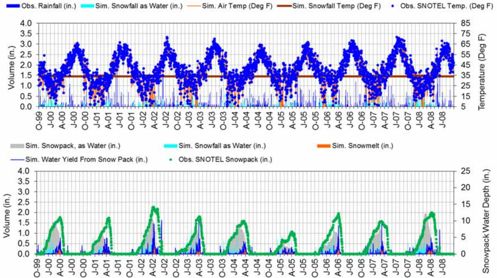
Figure F-31. LSPC snow calibration at WALDRON (South - 5600ft) (10/1/1999 - 9/30/2008).
