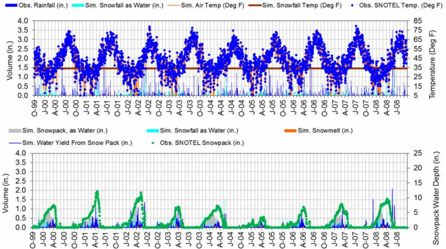
Figure F-5. LSPC snow calibration at DUPUYER CREEK (North - 5750ft) (10/1/1999 - 9/30/2008).
