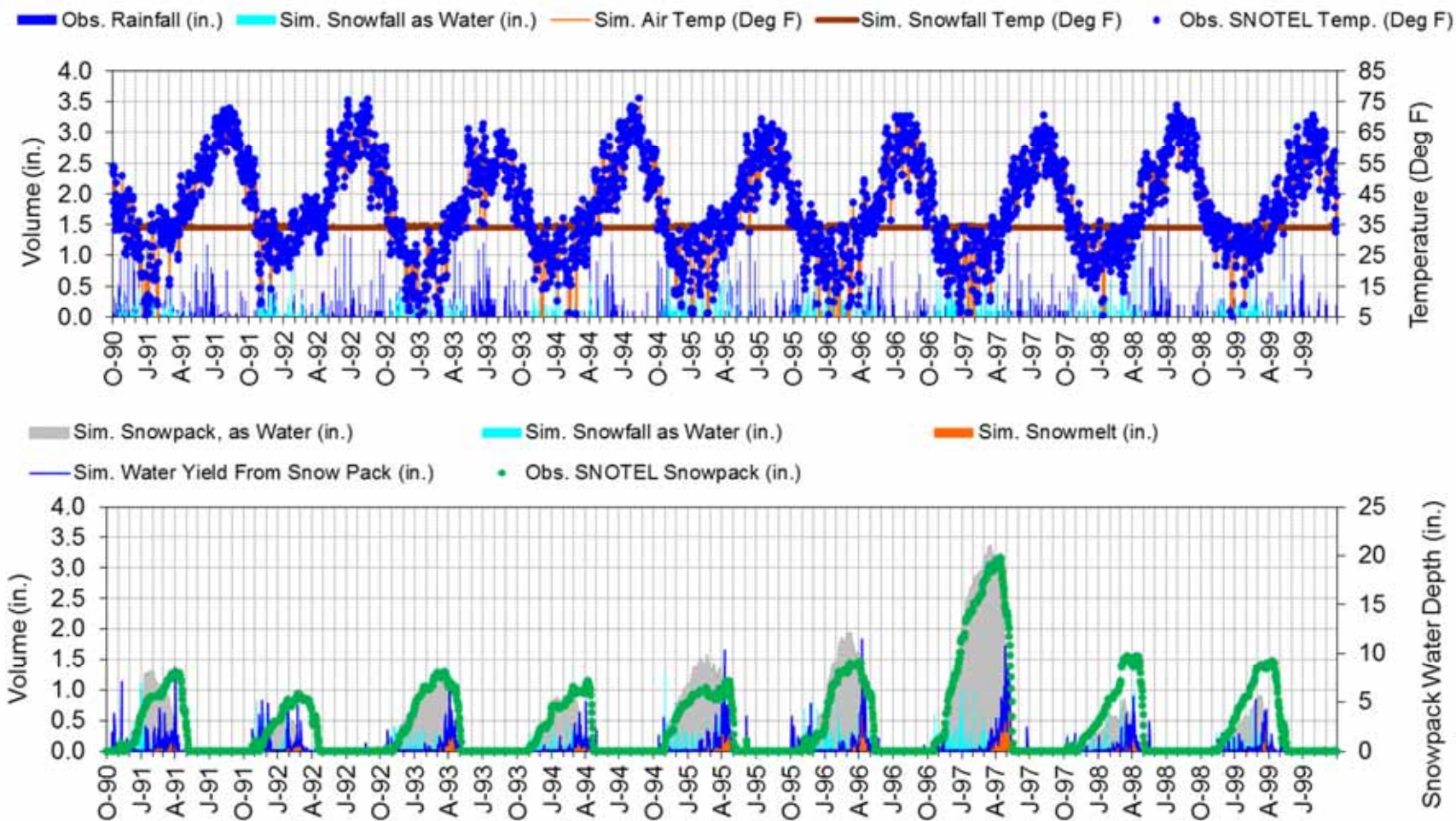
Figure F-4. LSPC snow calibration at BISSON CREEK (South - 4920ft) (10/1/1990 - 9/30/1999).
