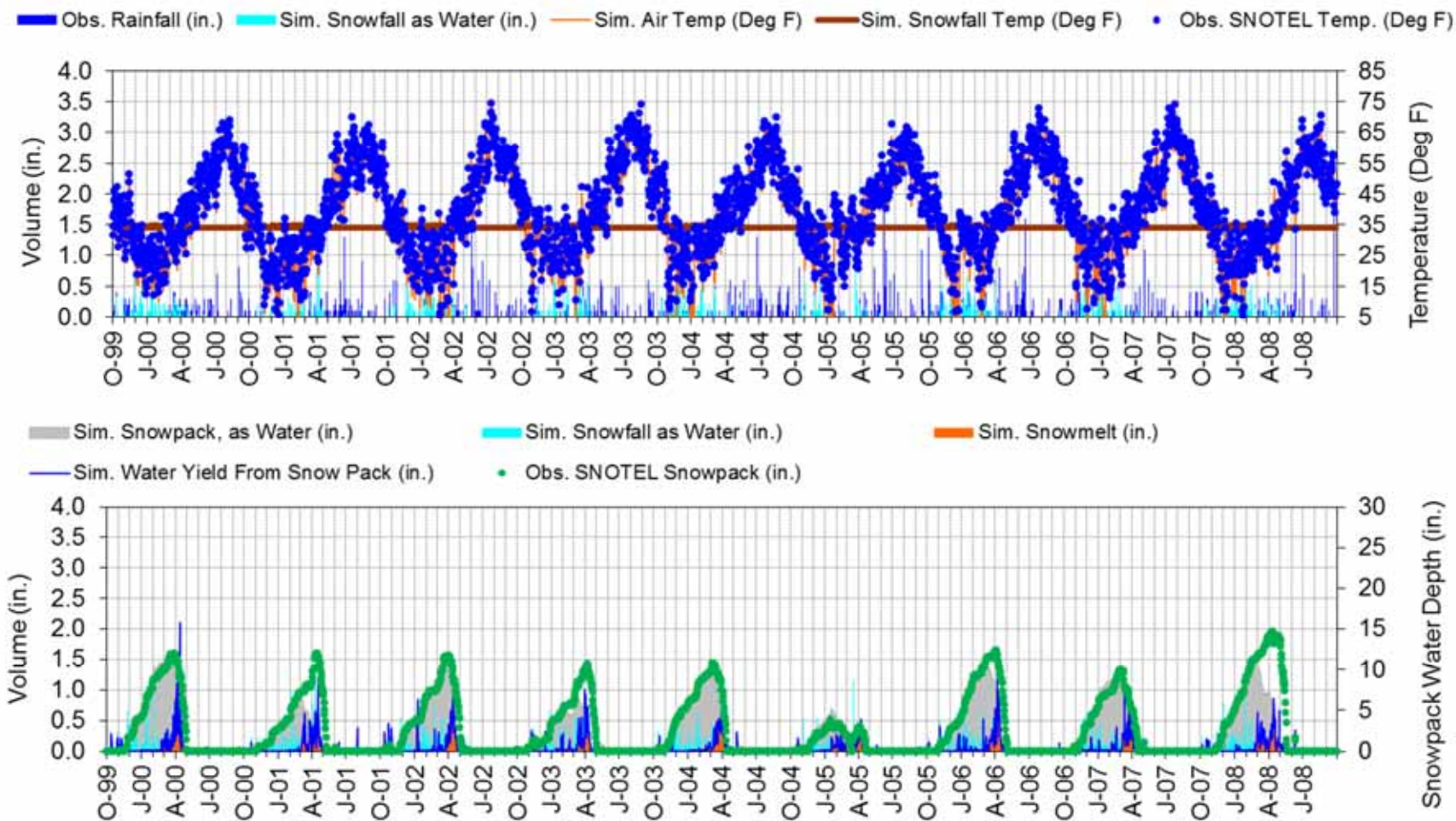
Figure F-13. LSPC snow calibration at HAND CREEK (North - 5035ft) (10/1/1999 - 9/30/2008).
