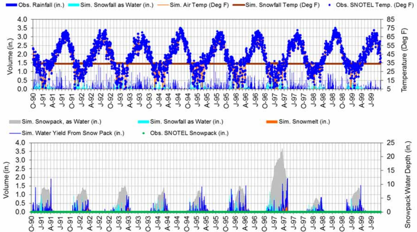
Figure F-16. LSPC snow calibration at KRAFT CREEK (South - 4750ft) (10/1/1990 - 9/30/1999).
