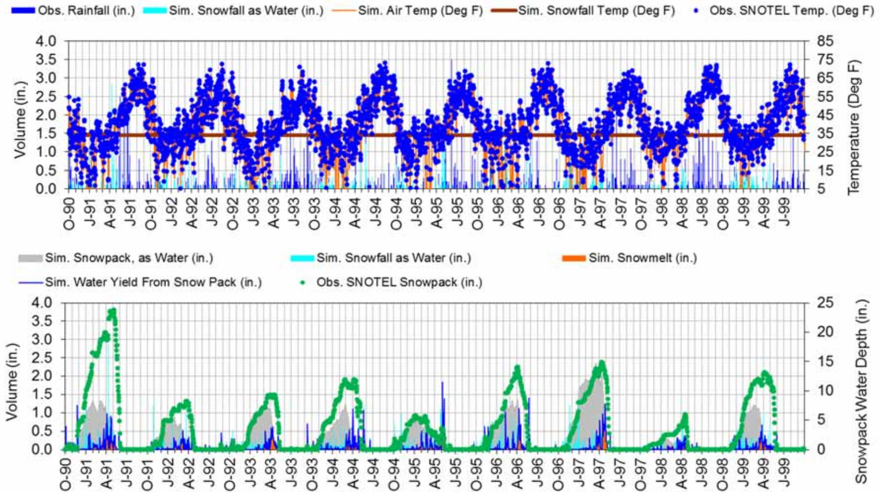
Figure F-6. LSPC snow calibration at DUPUYER CREEK (North - 5750ft) (10/1/1990 - 9/30/1999).
