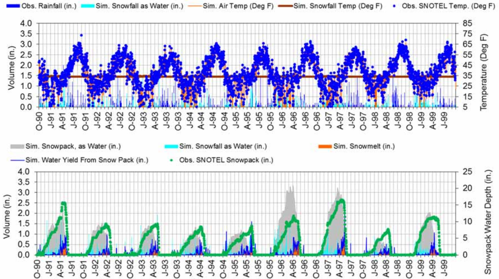
Figure F-34. LSPC snow calibration at WOOD CREEK (North - 5960ft) (10/1/1990 - 9/30/1999).
