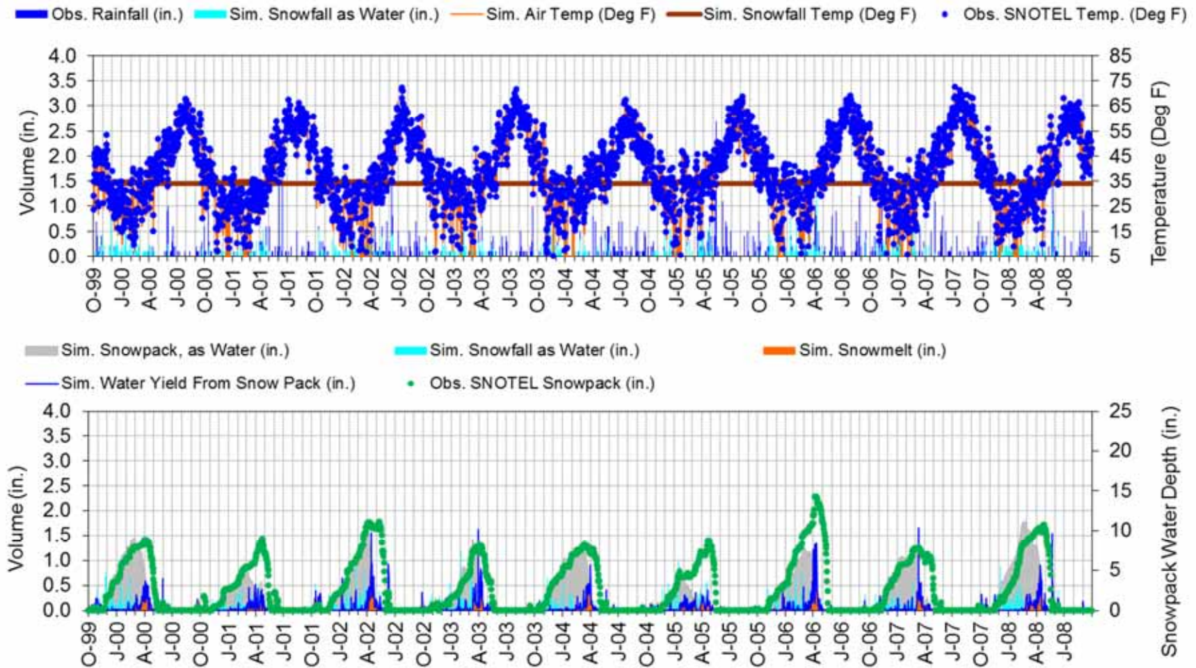
Figure F-33. LSPC snow calibration at WOOD CREEK (North - 5960ft) (10/1/1999 - 9/30/2008).
