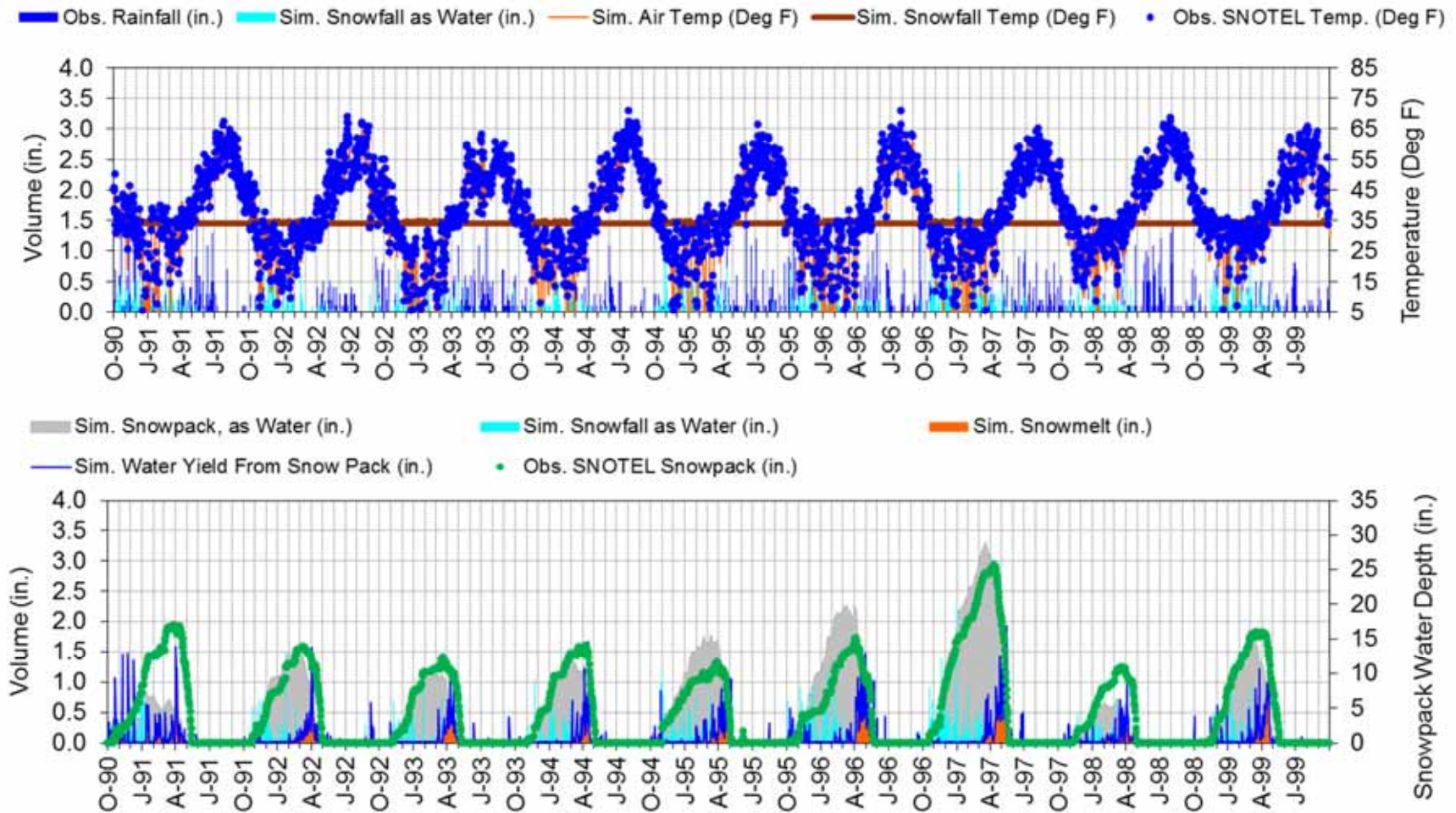
Figure F-8. LSPC snow calibration at EMERY CREEK (South - 4350ft) (10/1/1990 - 9/30/1999).
