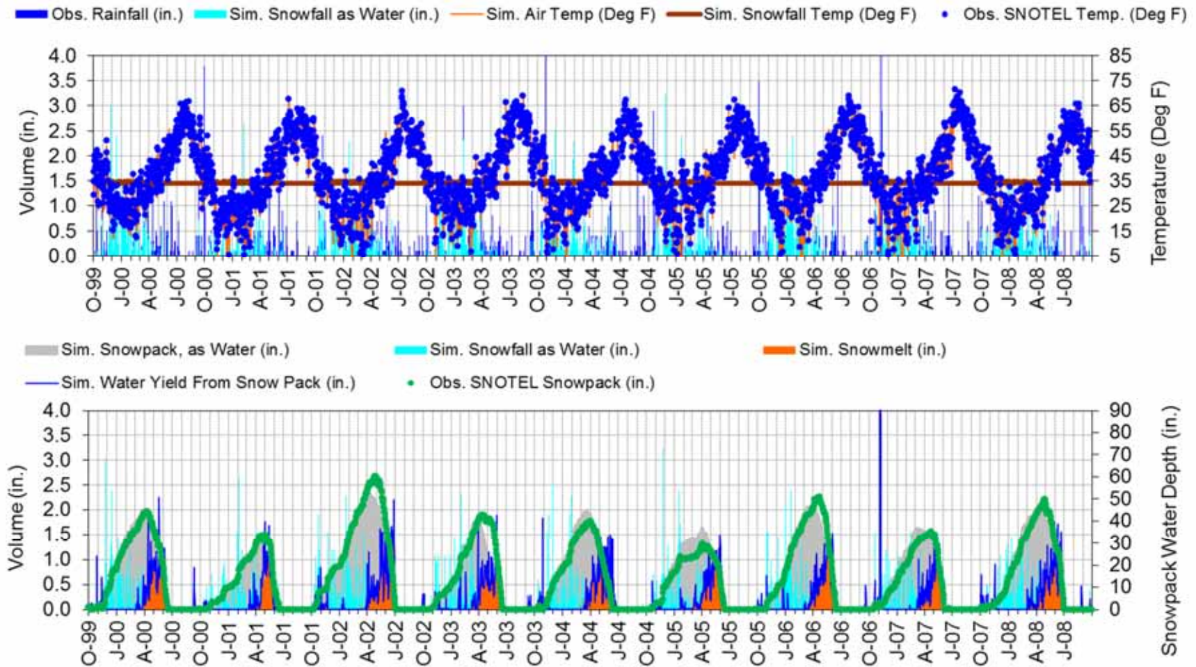
Figure F-25. LSPC snow calibration at NORTH FORK JOCKO (South - 6330ft) (10/1/1999 - 9/30/2008).
