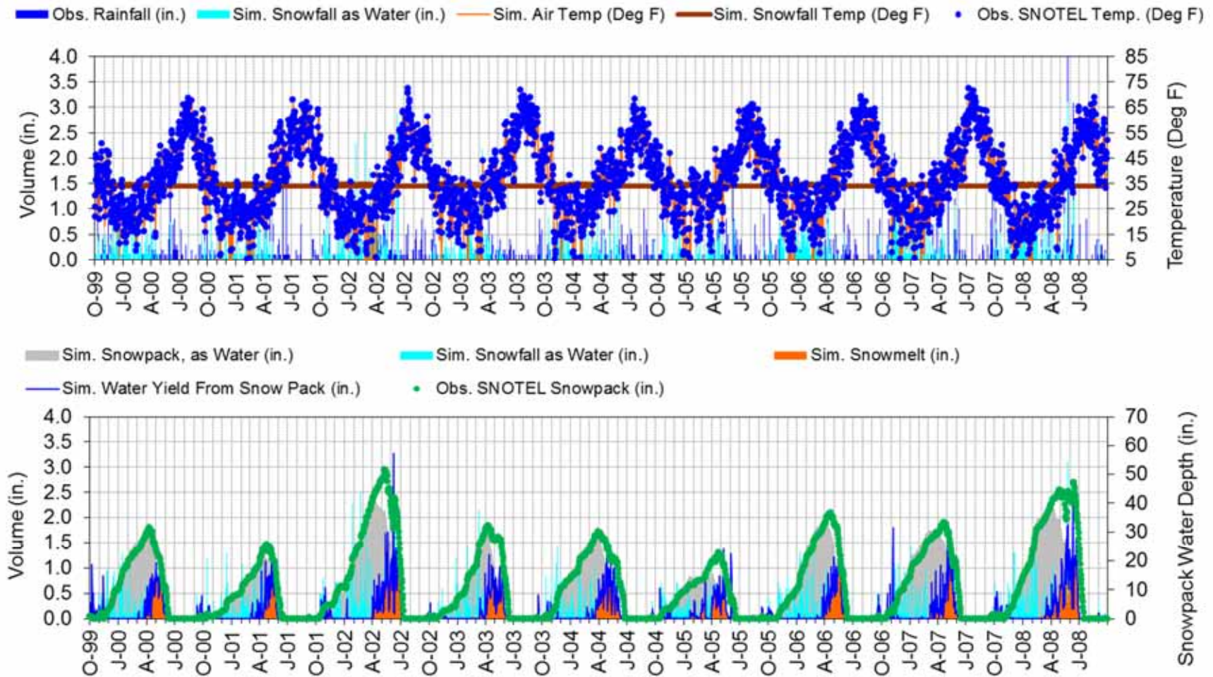
Figure F-1. LSPC snow calibration at BADGER PASS (South - 6900ft) (10/1/1999 - 9/30/2008).
