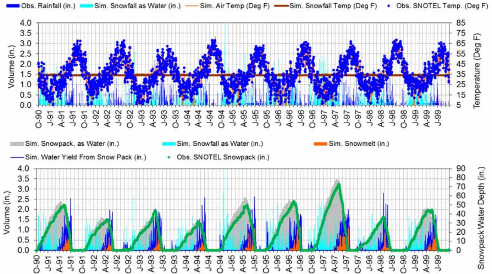
Figure F-20. LSPC snow calibration at MOSS PEAK (North - 6780ft) (10/1/1990 - 9/30/1999).
