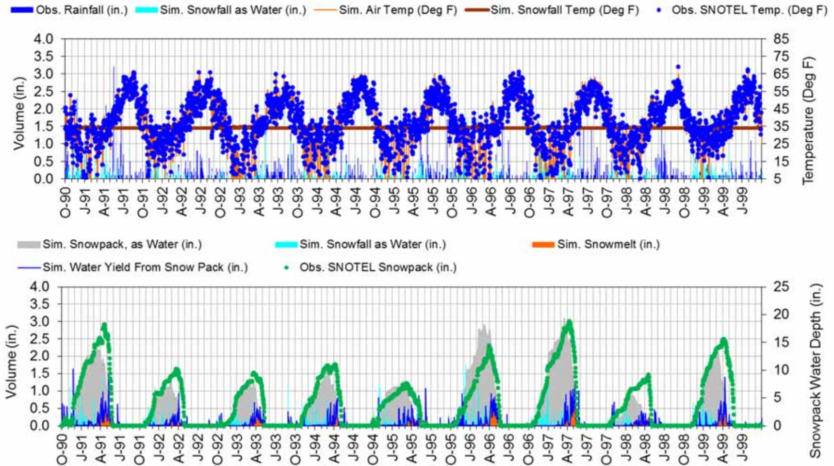
Figure F-32. LSPC snow calibration at WALDRON (South - 5600ft) (10/1/1990 - 9/30/1999).
