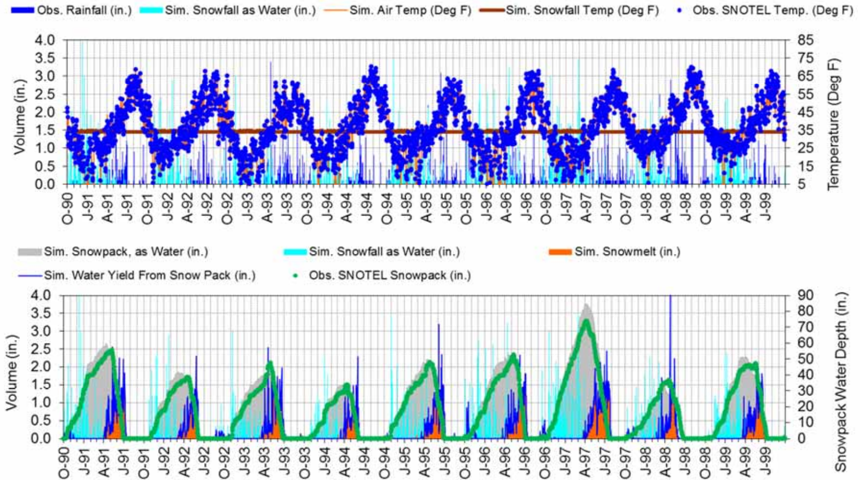
Figure F-24. LSPC snow calibration at NOISY BASIN (South - 6040ft) (10/1/1990 - 9/30/1999).
