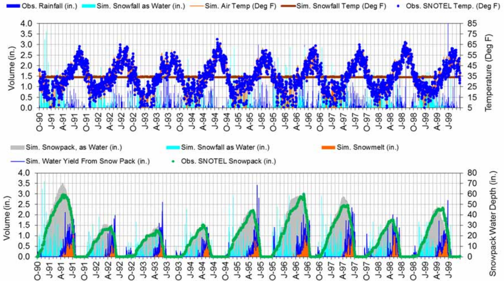
Figure F-30. LSPC snow calibration at STAHL PEAK (South - 6030ft) (10/1/1990 - 9/30/1999).
