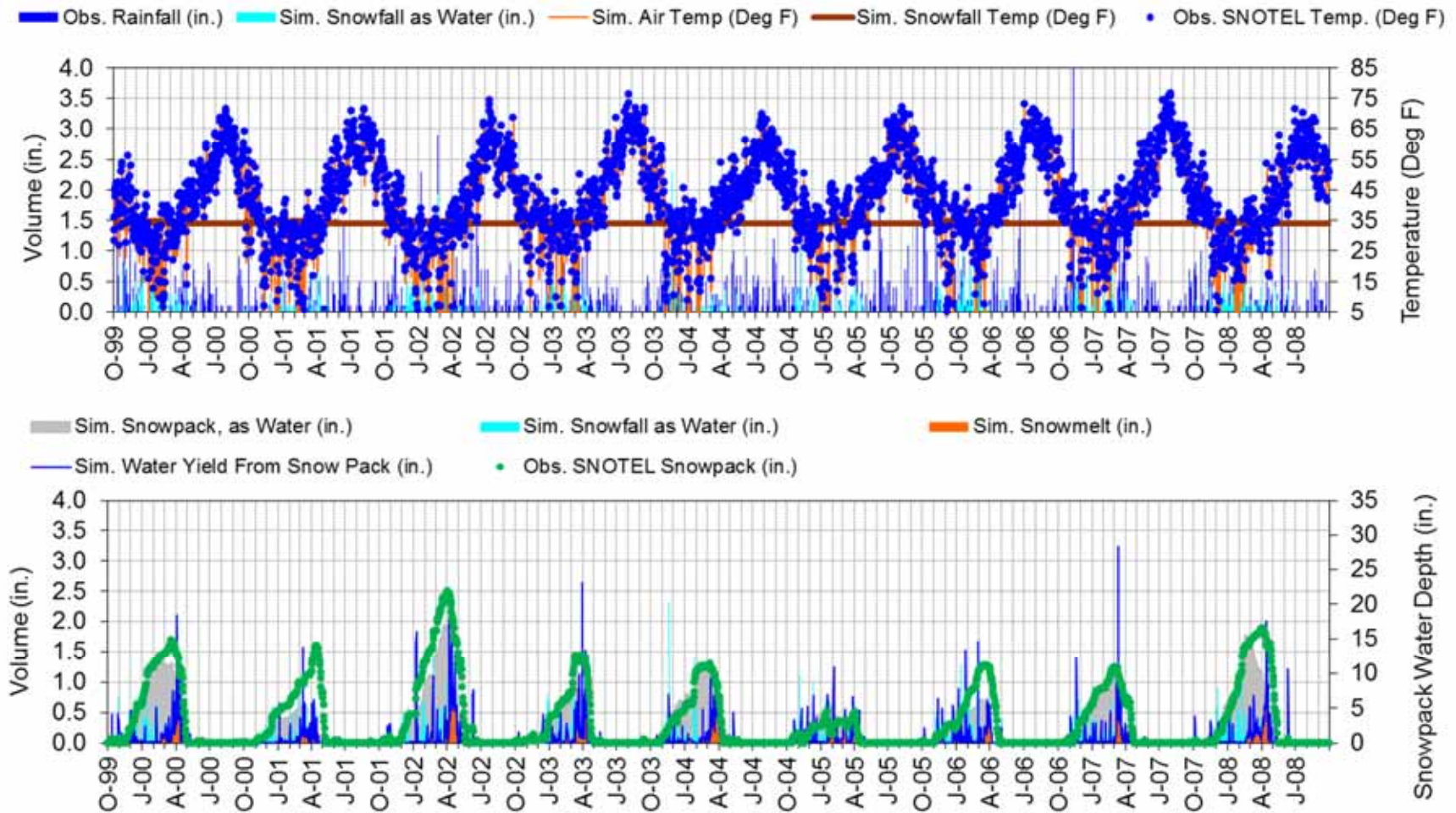
Figure F-17. LSPC snow calibration at MANY GLACIER (South - 4900ft) (10/1/1999 - 9/30/2008).
