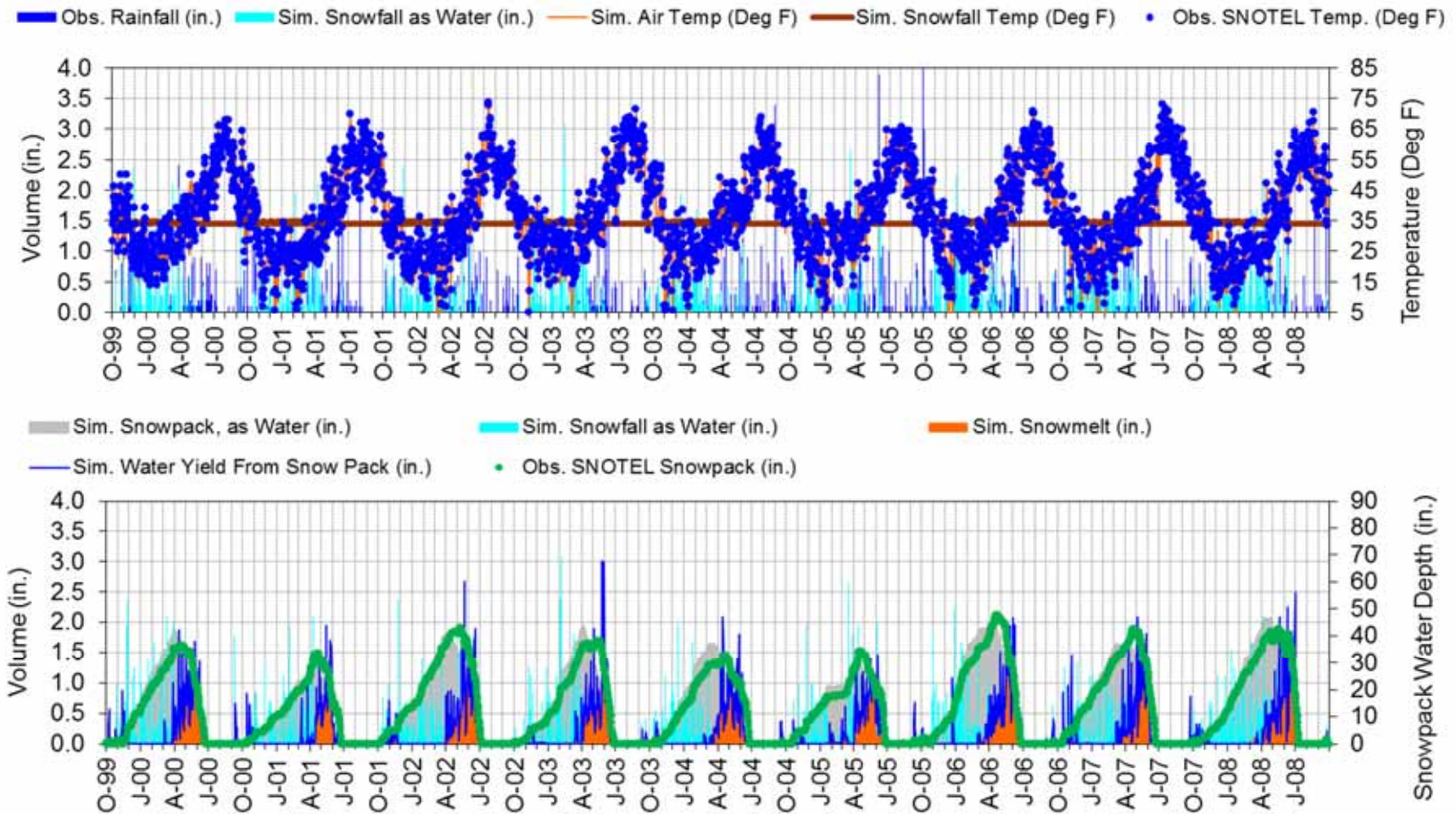
Figure F-19. LSPC snow calibration at MOSS PEAK (North - 6780ft) (10/1/1999 - 9/30/2008).
