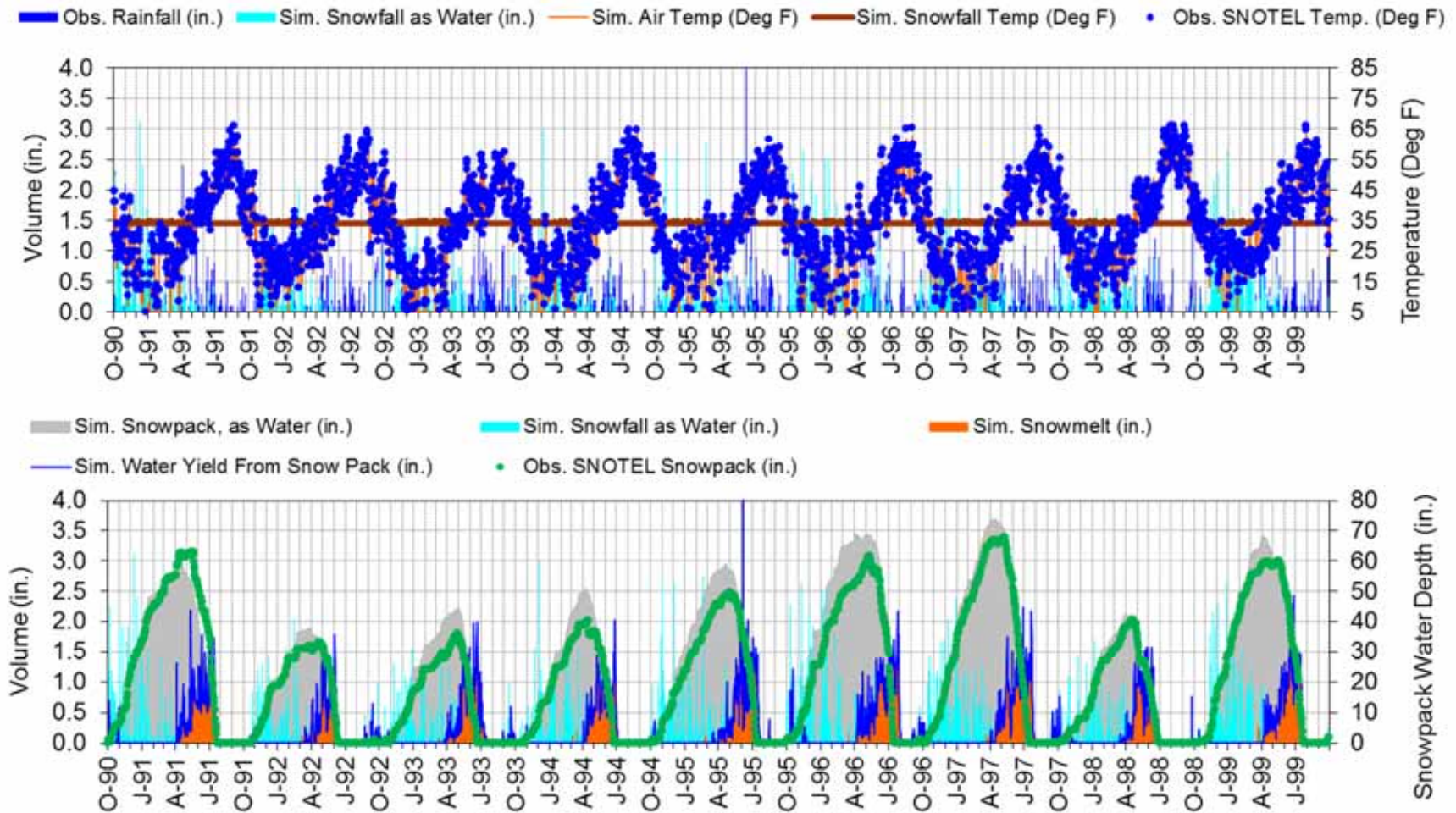
Figure F-10. LSPC snow calibration at FLATTOP MTN. (North - 6300ft) (10/1/1990 - 9/30/1999).
