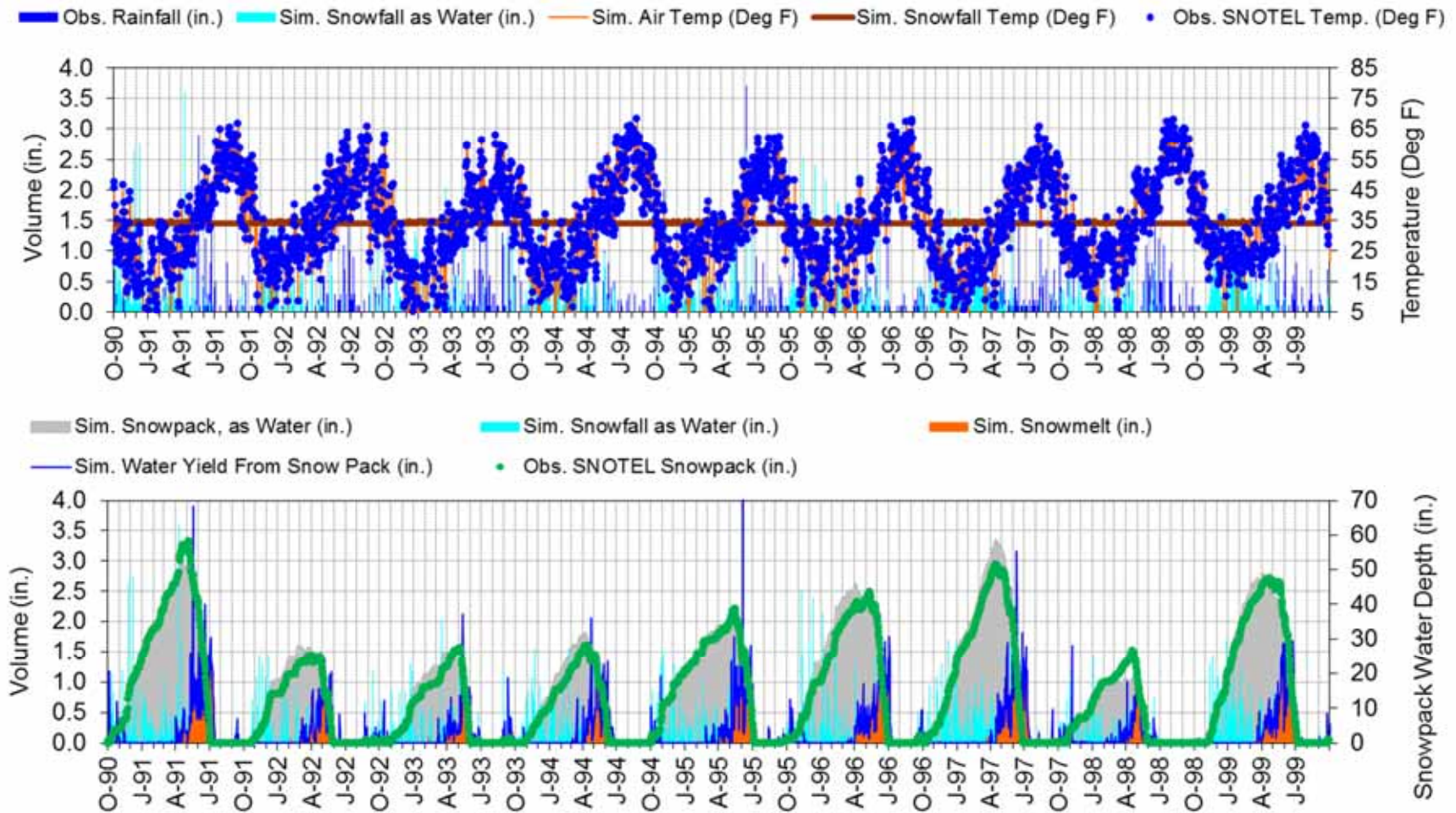
Figure F-2. LSPC snow calibration at BADGER PASS (South - 6900ft) (10/1/1990 - 9/30/1999).
