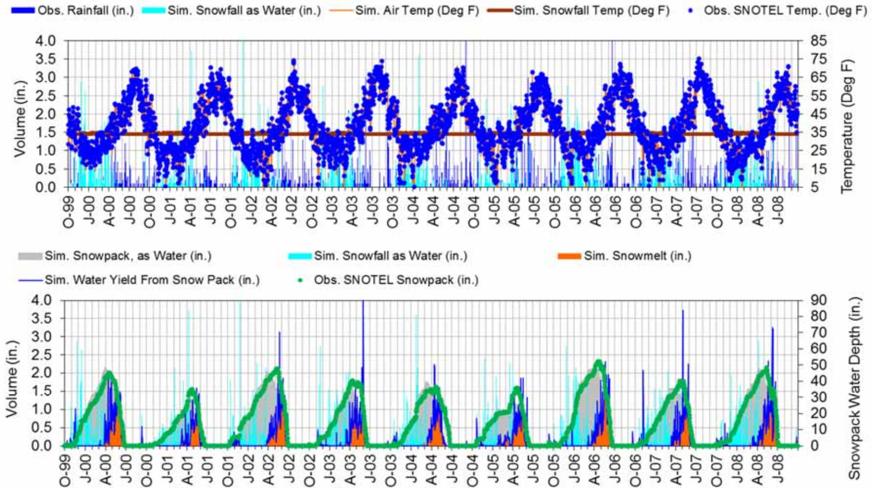
Figure F-23. LSPC snow calibration at NOISY BASIN (South - 6040ft) (10/1/1999 - 9/30/2008).
