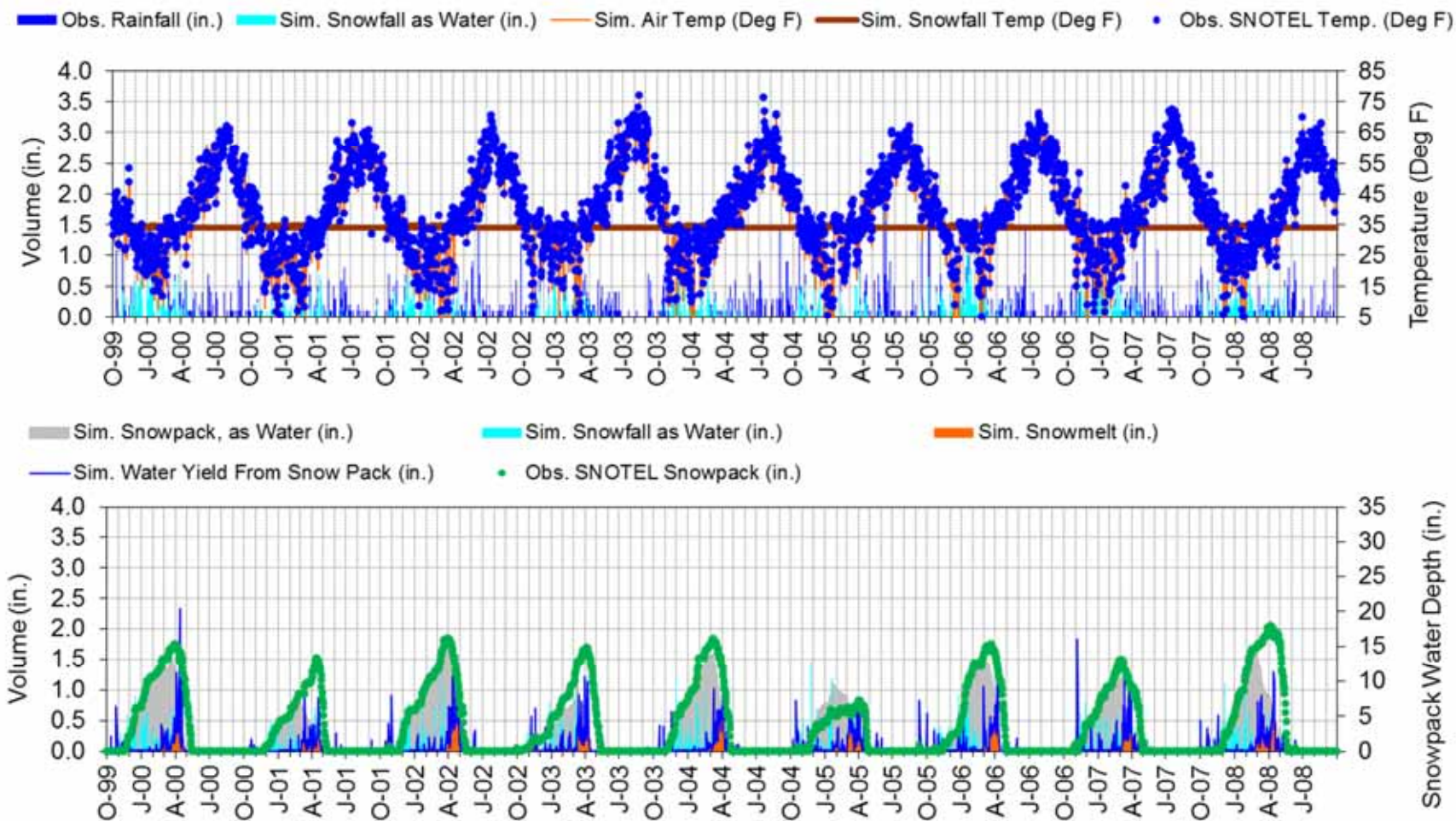
Figure F-7. LSPC snow calibration at EMERY CREEK (South - 4350ft) (10/1/1999 - 9/30/2008)
