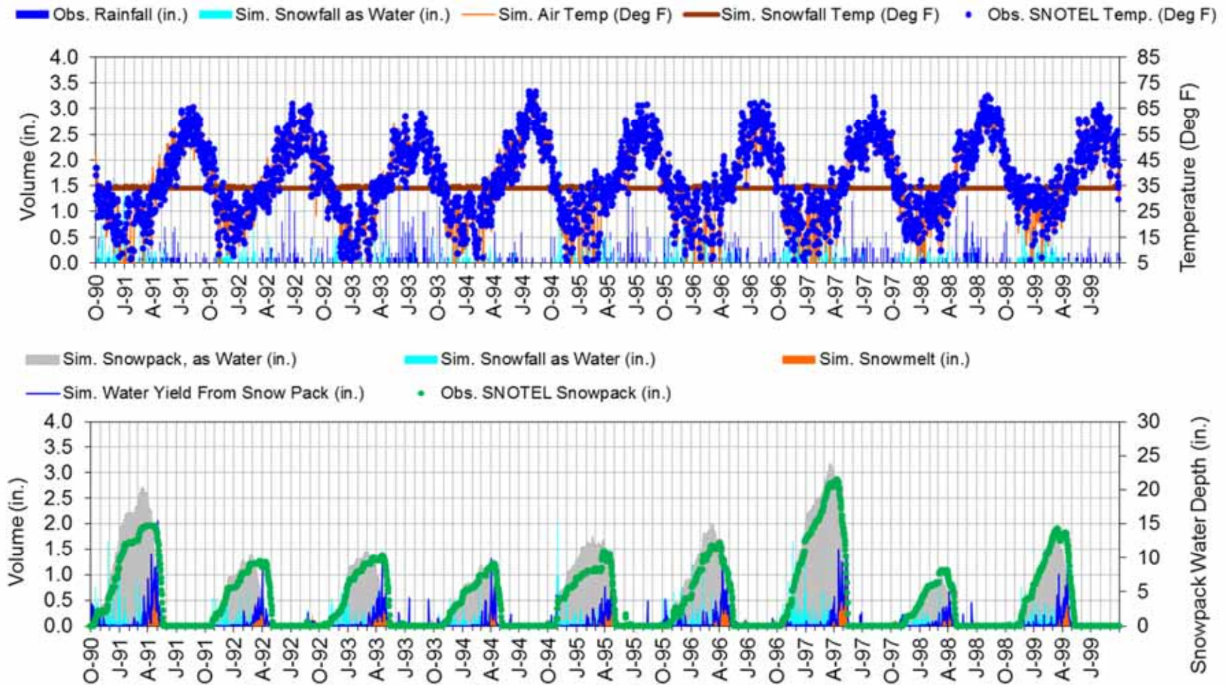
Figure F-14. LSPC snow calibration at HAND CREEK (North - 5035ft) (10/1/1990 - 9/30/1999).
