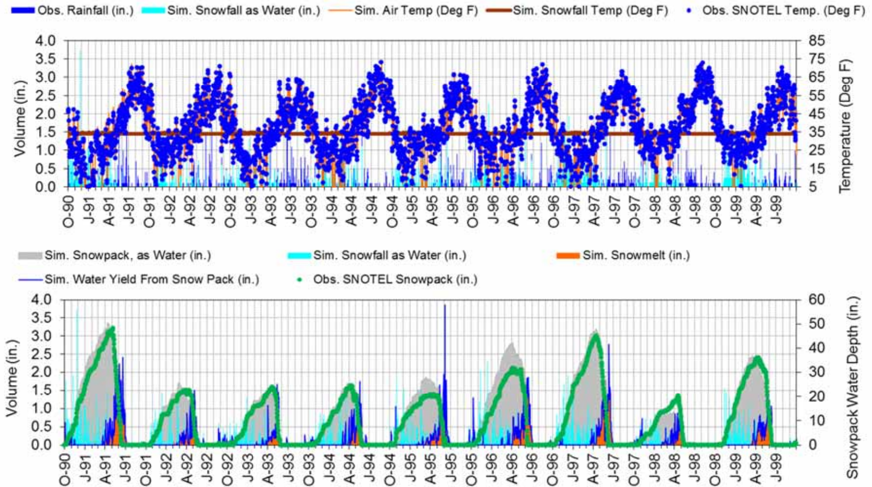
Figure F-28. LSPC snow calibration at PIKE CREEK (South - 5930ft) (10/1/1990 - 9/30/1999).
