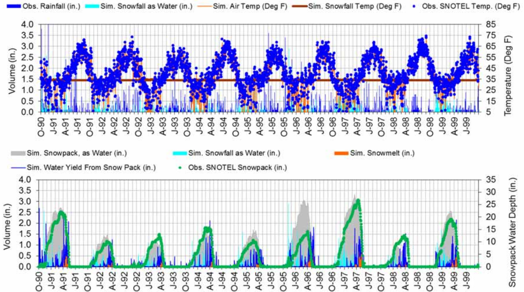
Figure F-18. LSPC snow calibration at MANY GLACIER (South - 4900ft) (10/1/1990 - 9/30/1999).
