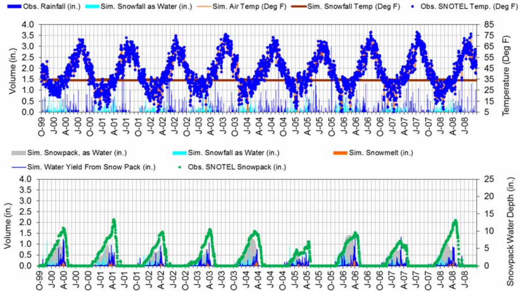
Figure F-3. LSPC snow calibration at BISSON CREEK (South - 4920ft) (10/1/1999 - 9/30/2008).
