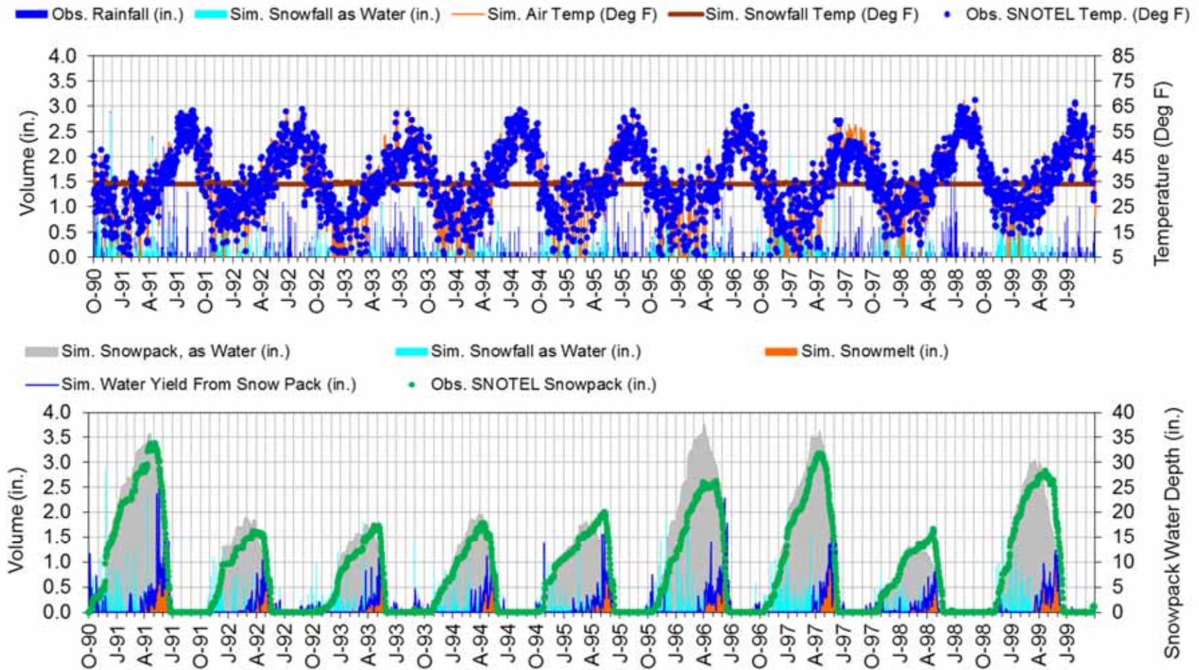
Figure F-22. LSPC snow calibration at MOUNT LOCKHART (North - 6400ft) (10/1/1990 - 9/30/1999).
