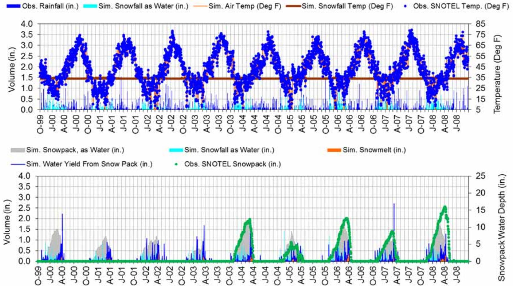
Figure F-15. LSPC snow calibration at KRAFT CREEK (South - 4750ft) (10/1/1999 - 9/30/2008).
