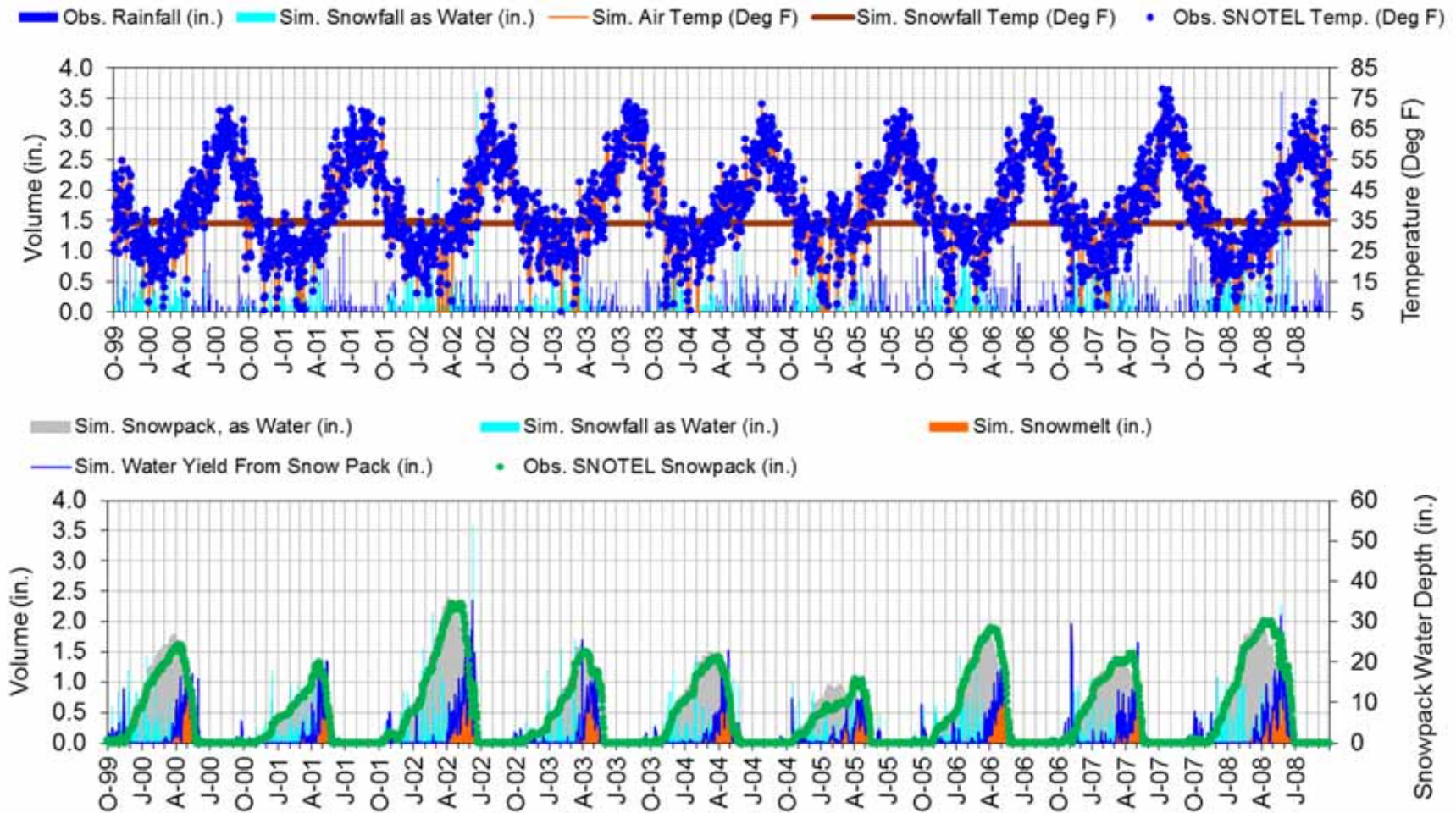
Figure F-27. LSPC snow calibration at PIKE CREEK (South - 5930ft) (10/1/1999 - 9/30/2008).
