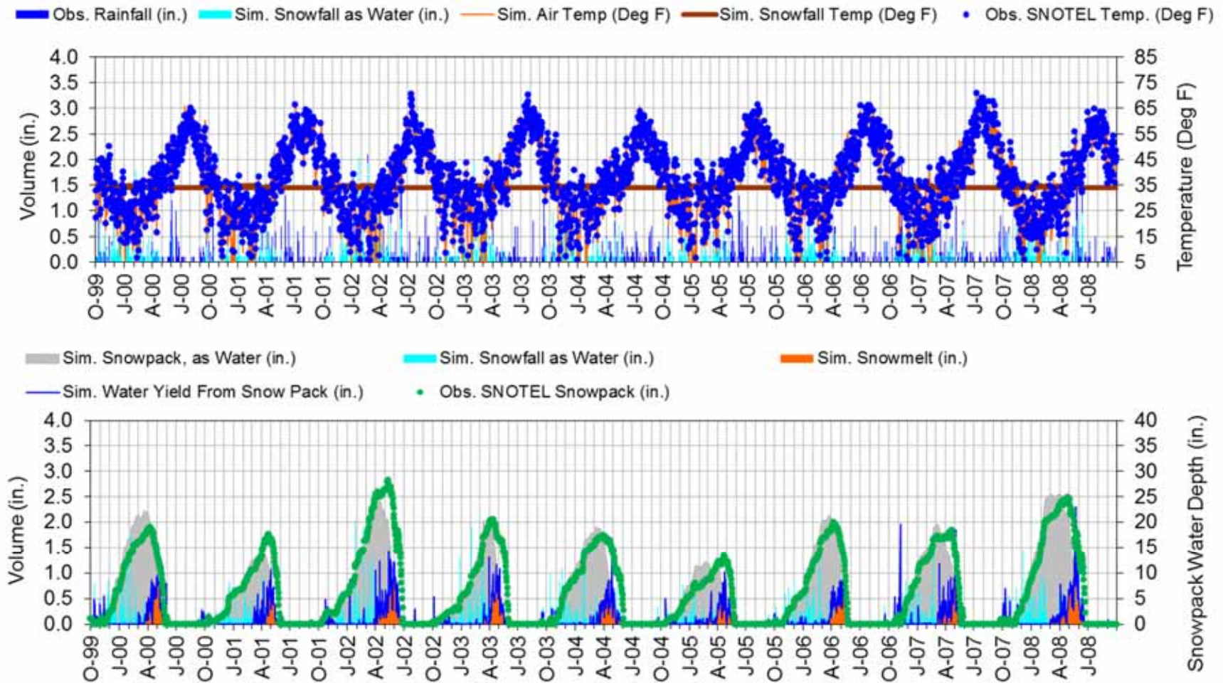
Figure F-21. LSPC snow calibration at MOUNT LOCKHART (North - 6400ft) (10/1/1999 - 9/30/2008).
