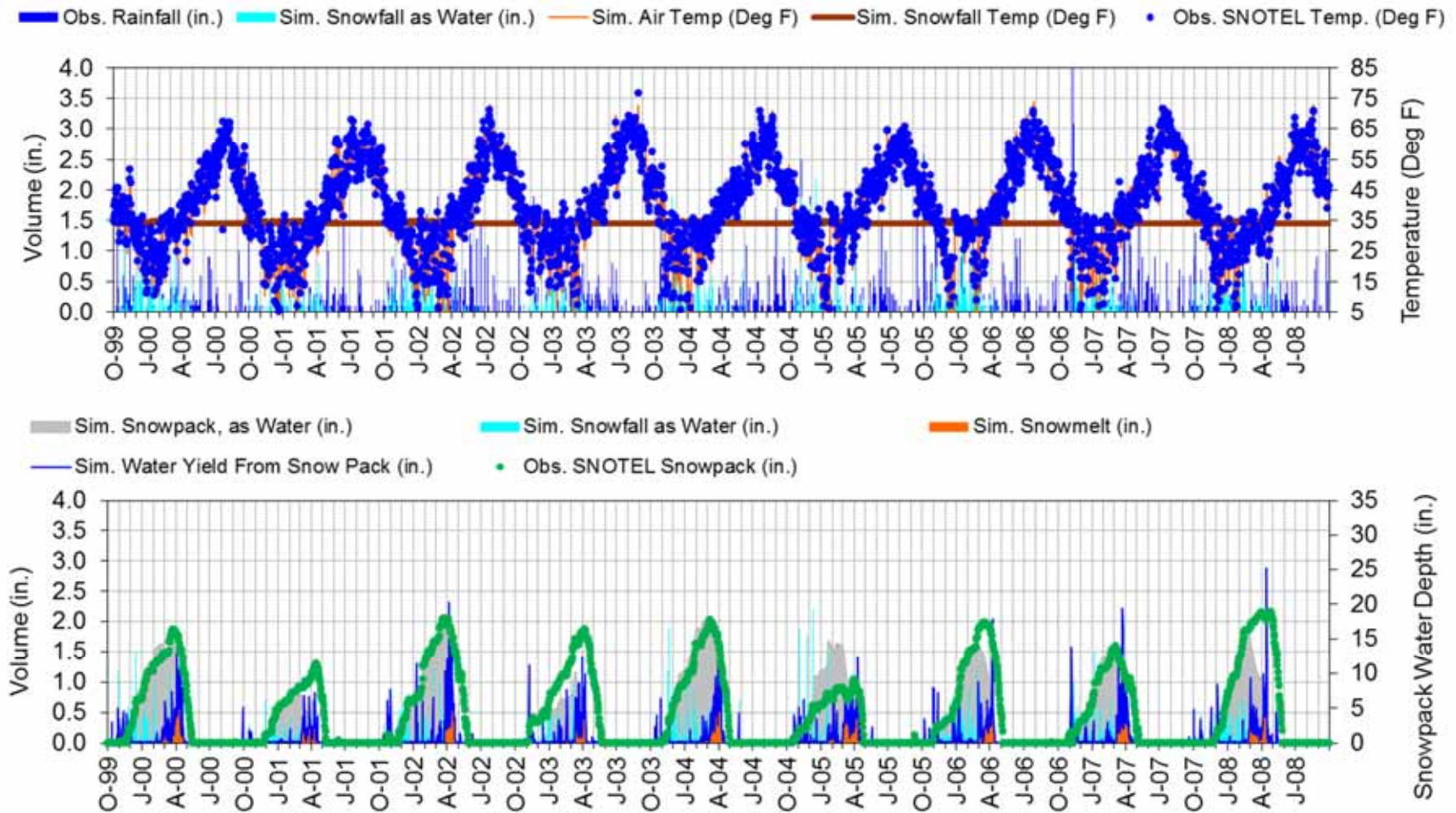
Figure F-11. LSPC snow calibration at GRAVE CREEK (North - 4300ft) (10/1/1999 - 9/30/2008).
