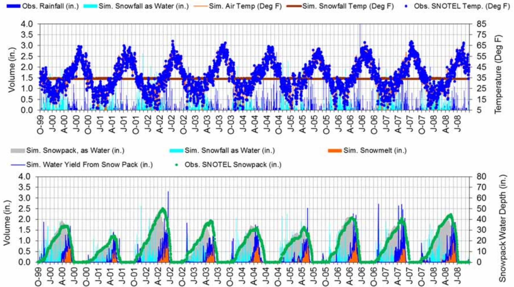
Figure F-29. LSPC snow calibration at STAHL PEAK (South - 6030ft) (10/1/1999 - 9/30/2008).
