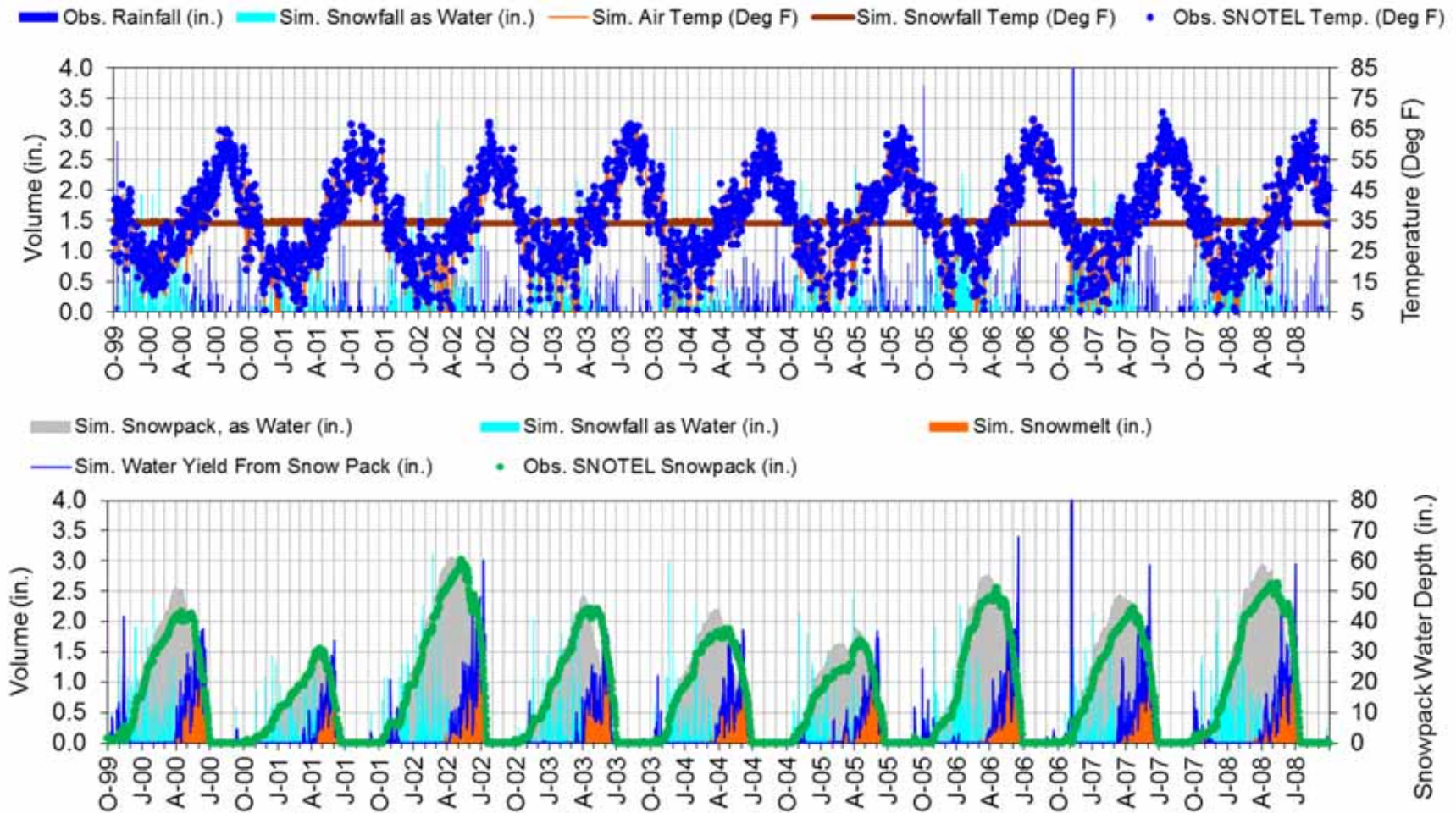
Figure F-9. LSPC snow calibration at FLATTOP MTN. (North - 6300ft) (10/1/1999 - 9/30/2008).
