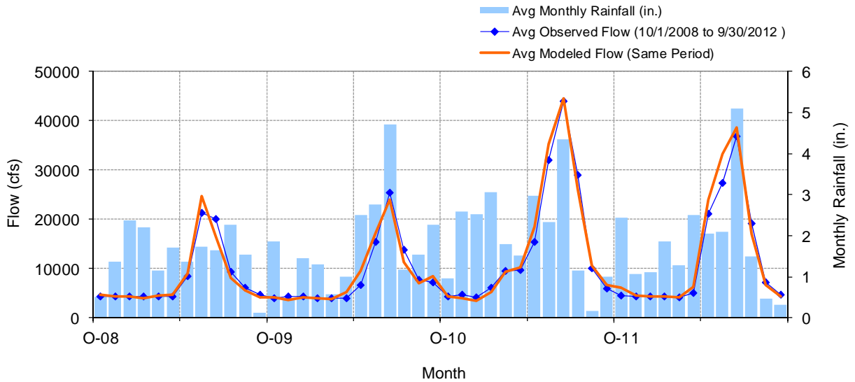
Figure G-32. Calibration Time Series of Observed and Modeled Monthly Flows and Monthly Rainfall, USGS 12369000 Flathead River near Bigfork, MT
