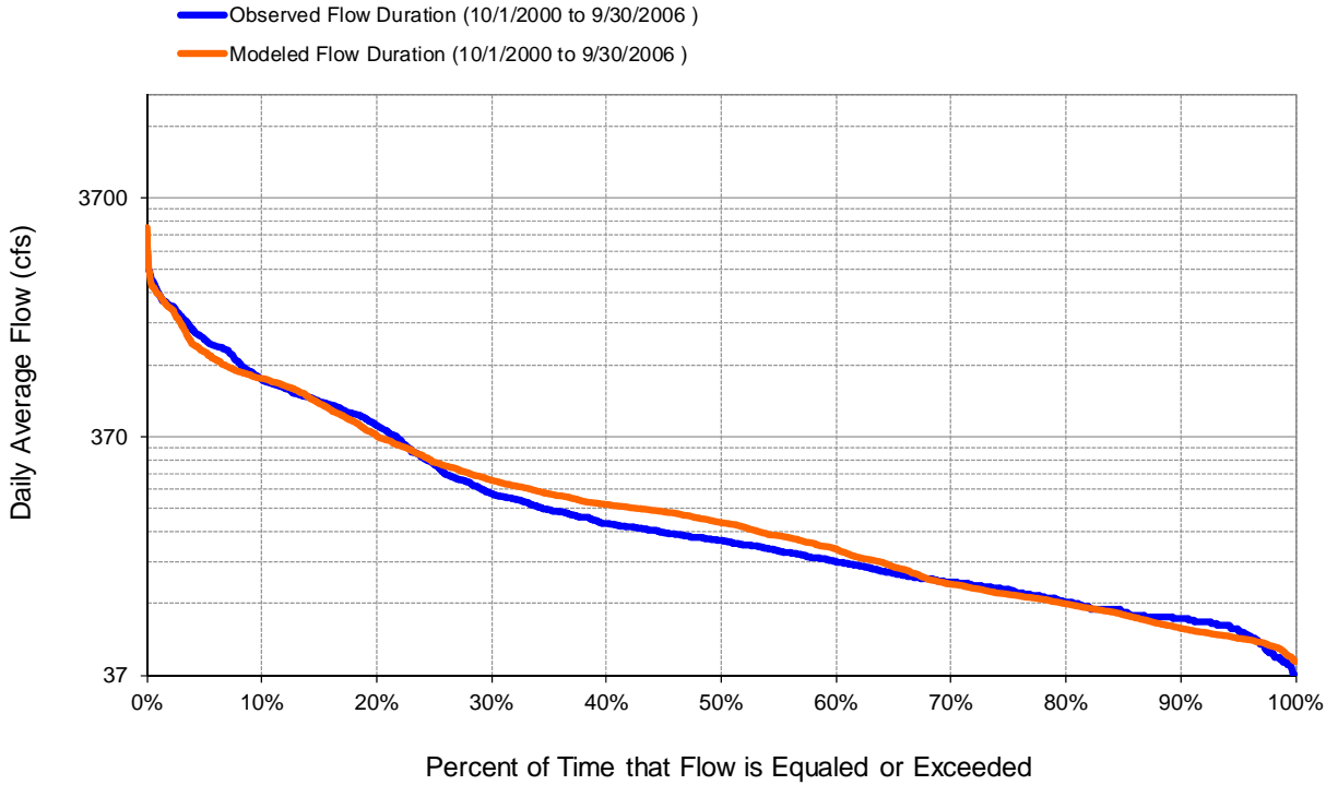
Figure G-21. Calibration Observed and Modeled Flow-Duration, USGS 12365000 Stillwater River near Whitefish, MT
