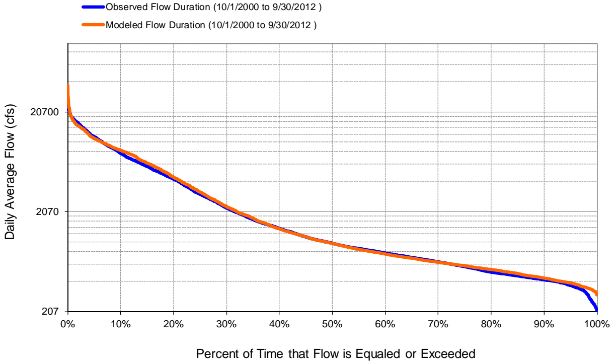
Figure G-11. Calibration Observed and Modeled Flow-Duration, USGS 12358500 M F Flathead River near West Glacier, MT
