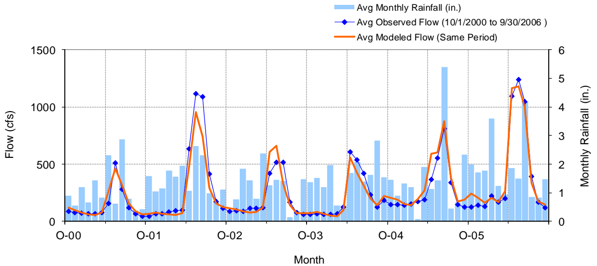
Figure G-22. Calibration Time Series of Observed and Modeled Monthly Flows and Monthly Rainfall, USGS 12365000 Stillwater River near Whitefish, MT
