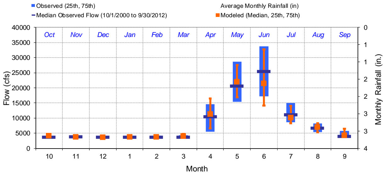
Figure G-19. Calibration Observed and Modeled Monthly Flow Distributions with Monthly Rainfall, USGS 12363000 Flathead River at Columbia Falls, MT
