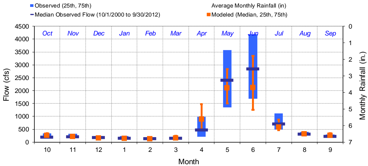
Figure G-4. Calibration Observed and Modeled Monthly Flow Distributions with Monthly Rainfall, USGS 12355000 Flathead River at Flathead, BC
