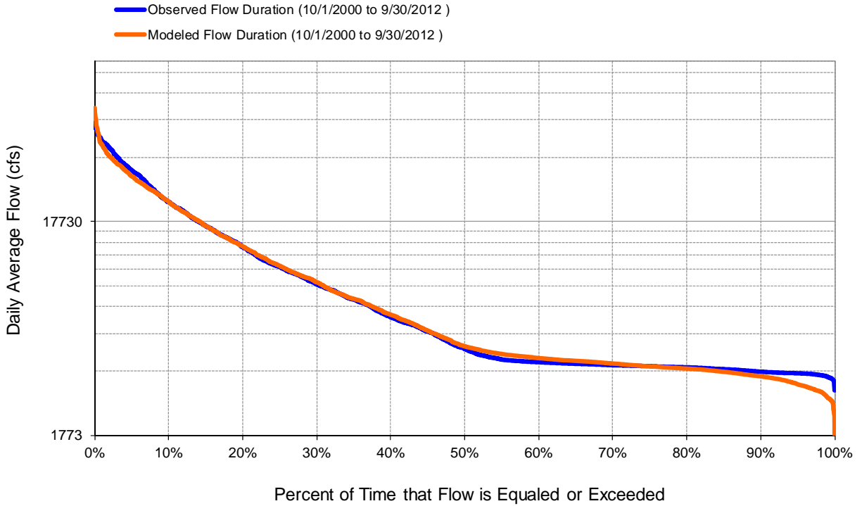
Figure G-16. Calibration Observed and Modeled Flow-Duration, USGS 12363000 Flathead River at Columbia Falls, MT
