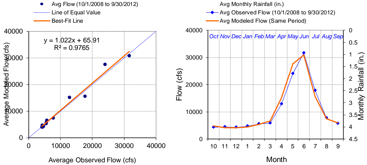
Figure G-35. Calibration Observed and Modeled Monthly Average Flow with Monthly Rainfall, USGS 12369000 Flathead River near Bigfork, MT
