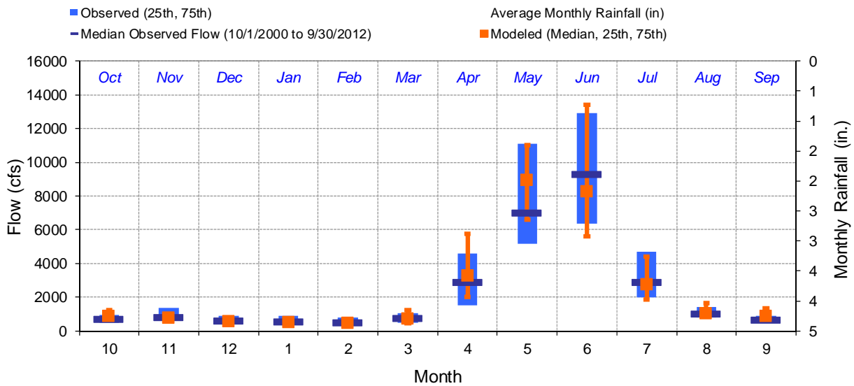
Figure G-14. Calibration Observed and Modeled Monthly Flow Distributions with Monthly Rainfall, USGS 12358500 M F Flathead River near West Glacier, MT
