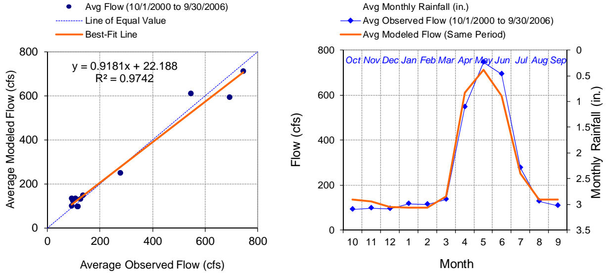
Figure G-25. Calibration Observed and Modeled Monthly Average Flow with Monthly Rainfall, USGS 12365000 Stillwater River near Whitefish, MT
