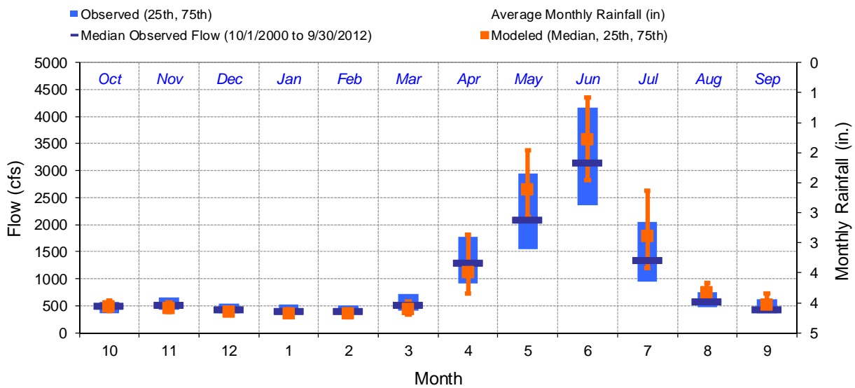
Figure G-39. Calibration Observed and Modeled Monthly Flow Distributions with Monthly Rainfall, USGS 12370000 Swan River near Bigfork, MT
