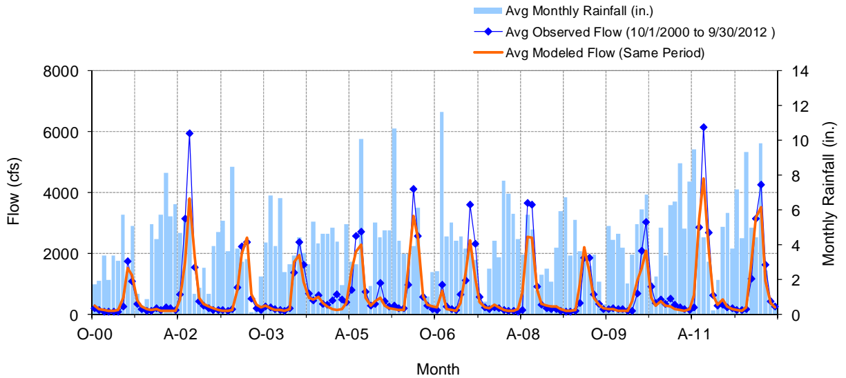
Figure G-2. Calibration Time Series of Observed and Modeled Monthly Flows and Monthly Rainfall, USGS 12355000 Flathead River at Flathead, BC
