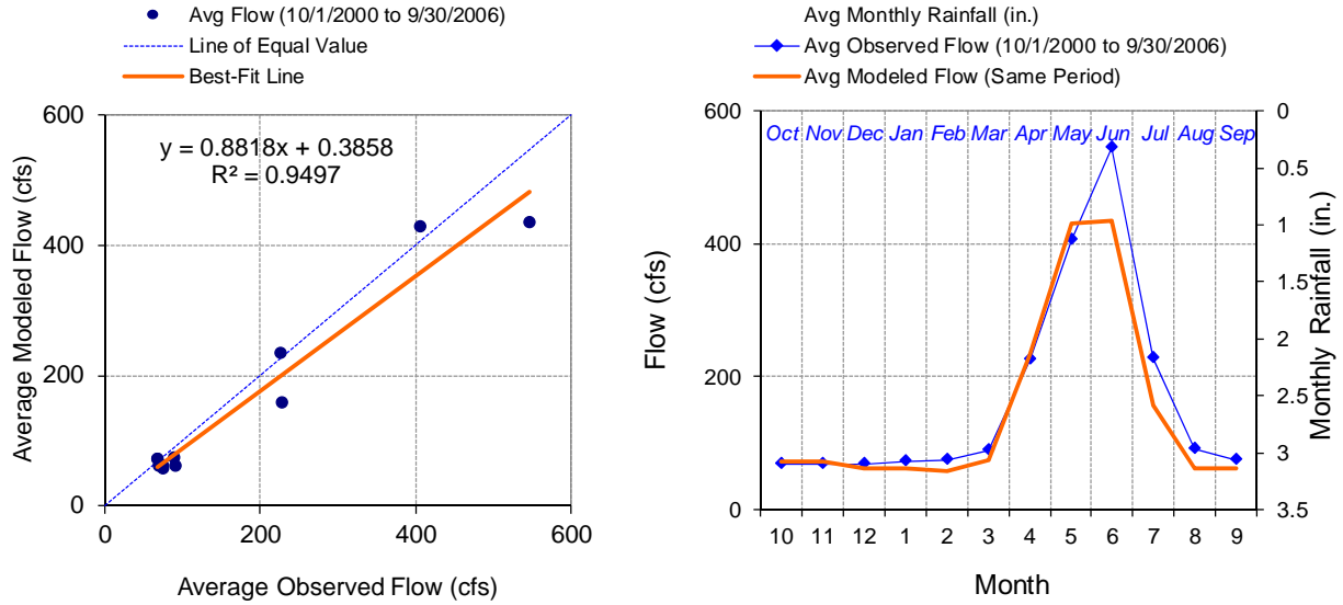
Figure G-30. Calibration Observed and Modeled Monthly Average Flow with Monthly Rainfall, USGS 12366000 Whitefish River near Kalispell, MT
