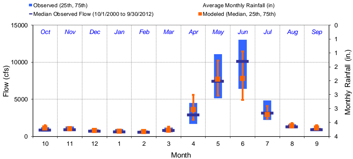
Figure G-9. Calibration Observed and Modeled Monthly Flow Distributions with Monthly Rainfall, USGS 12355500 N F Flathead River nr Columbia Falls, MT
