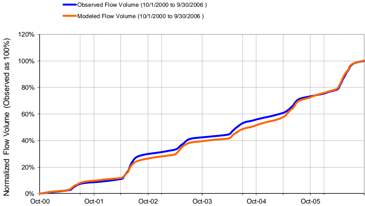
Figure G-23. Calibration Cumulative Observed and Modeled Flow Volume, USGS 12365000 Stillwater River near Whitefish, MT
