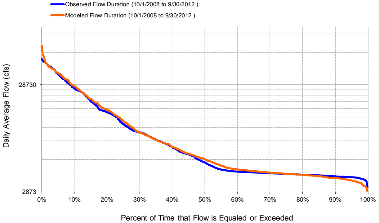
Figure G-31. Calibration Observed and Modeled Flow-Duration, USGS 12369000 Flathead River near Bigfork, MT
