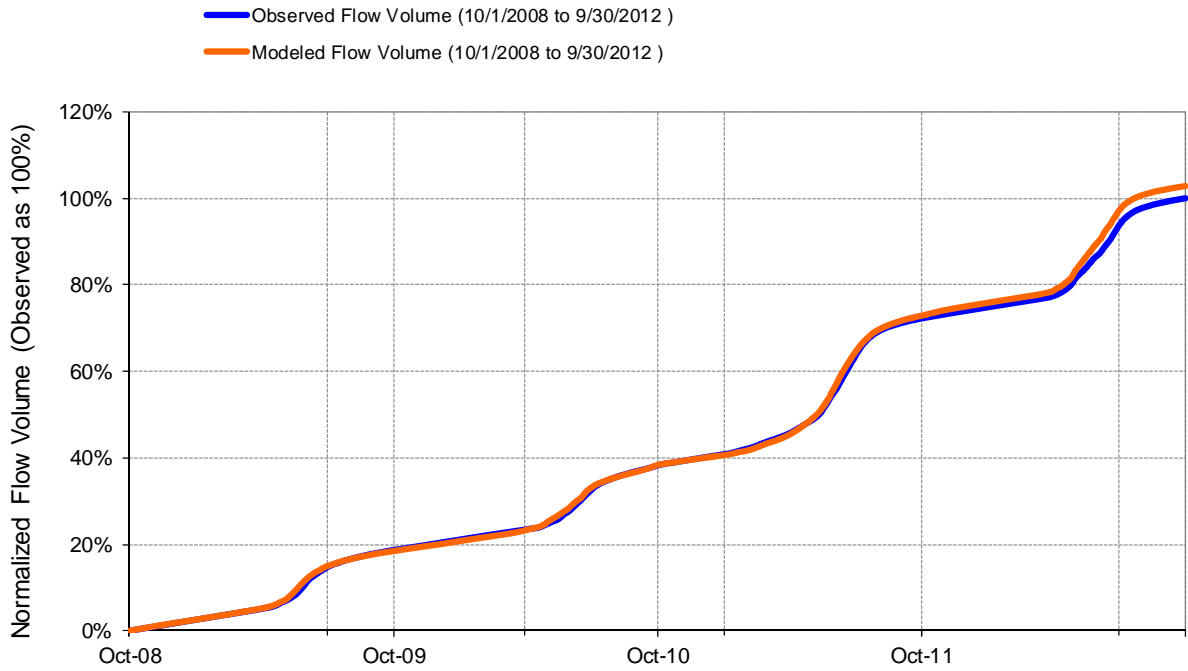
Figure G-33. Calibration Cumulative Observed and Modeled Flow Volume, USGS 12369000 Flathead River near Bigfork, MT
