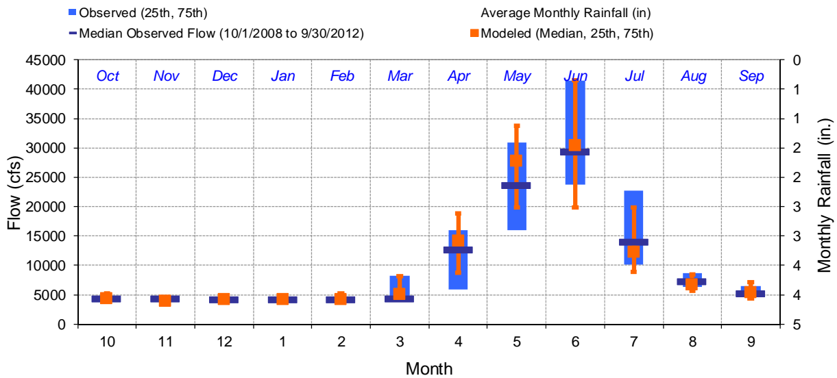
Figure G-34. Calibration Observed and Modeled Monthly Flow Distributions with Monthly Rainfall, USGS 12369000 Flathead River near Bigfork, MT
