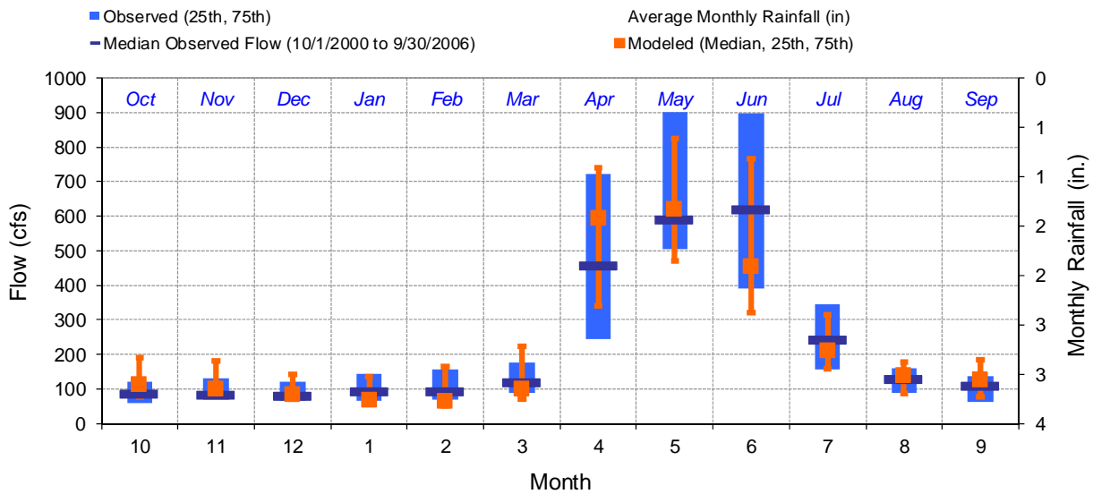
Figure G-24. Calibration Observed and Modeled Monthly Flow Distributions with Monthly Rainfall, USGS 12365000 Stillwater River near Whitefish, MT
