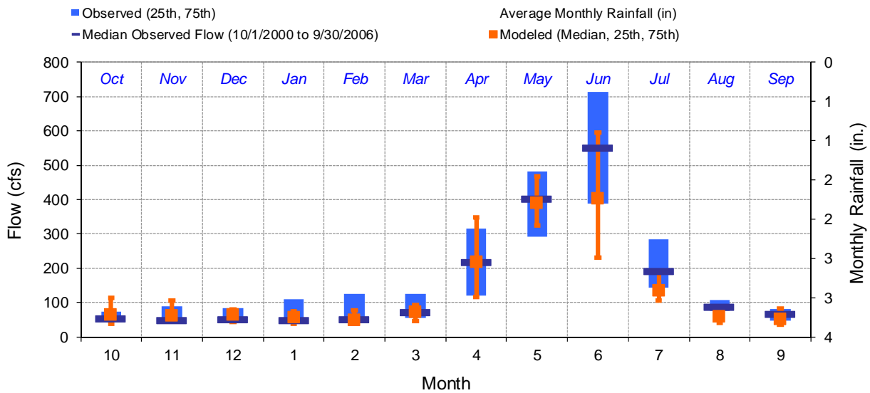
Figure G-29. Calibration Observed and Modeled Monthly Flow Distributions with Monthly Rainfall, USGS 12366000 Whitefish River near Kalispell, MT
