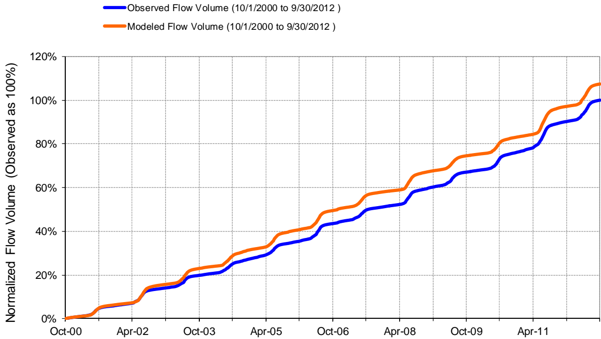
Figure G-38. Calibration Cumulative Observed and Modeled Flow Volume, USGS 12370000 Swan River near Bigfork, MT
