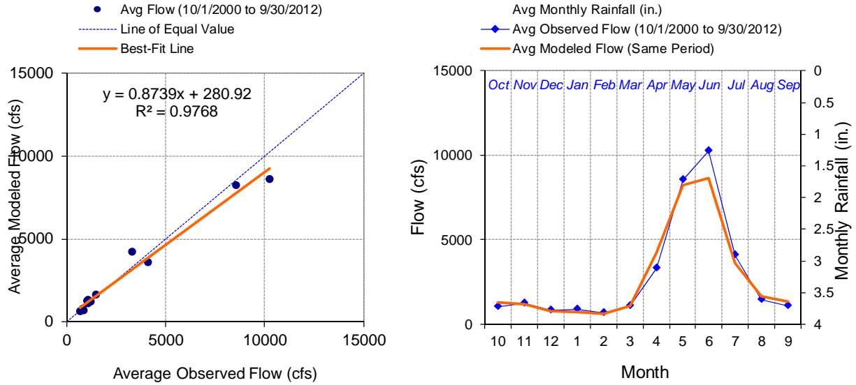
Figure G-10. Calibration Observed and Modeled Monthly Average Flow with Monthly Rainfall, USGS 12355500 N F Flathead River nr Columbia Falls, MT
