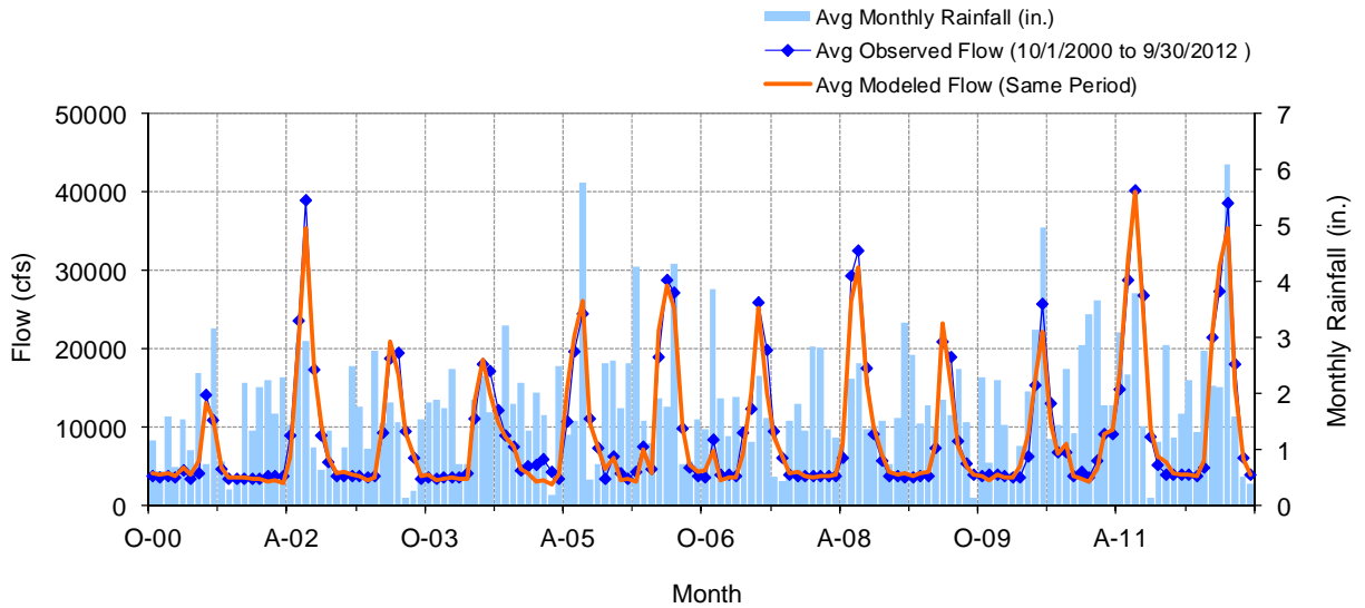
Figure G-17. Calibration Time Series of Observed and Modeled Monthly Flows and Monthly Rainfall, USGS 12363000 Flathead River at Columbia Falls, MT
