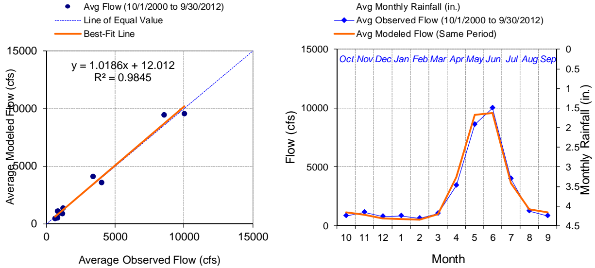
Figure G-15. Calibration Observed and Modeled Monthly Average Flow with Monthly Rainfall, USGS 12358500 M F Flathead River near West Glacier, MT
