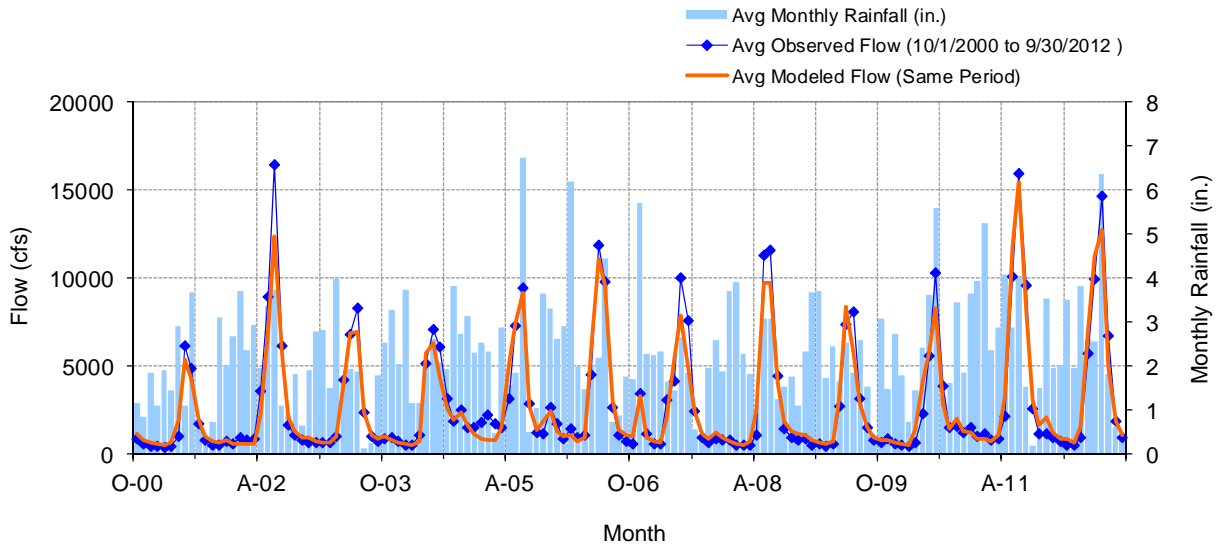
Figure G-7. Calibration Time Series of Observed and Modeled Monthly Flows and Monthly Rainfall, USGS 12355500 N F Flathead River nr Columbia Falls, MT
