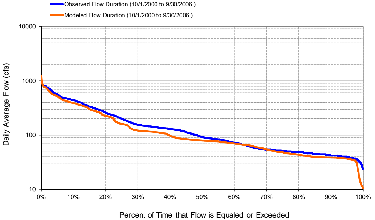
Figure G-26. Calibration Observed and Modeled Flow-Duration, USGS 12366000 Whitefish River near Kalispell, MT
