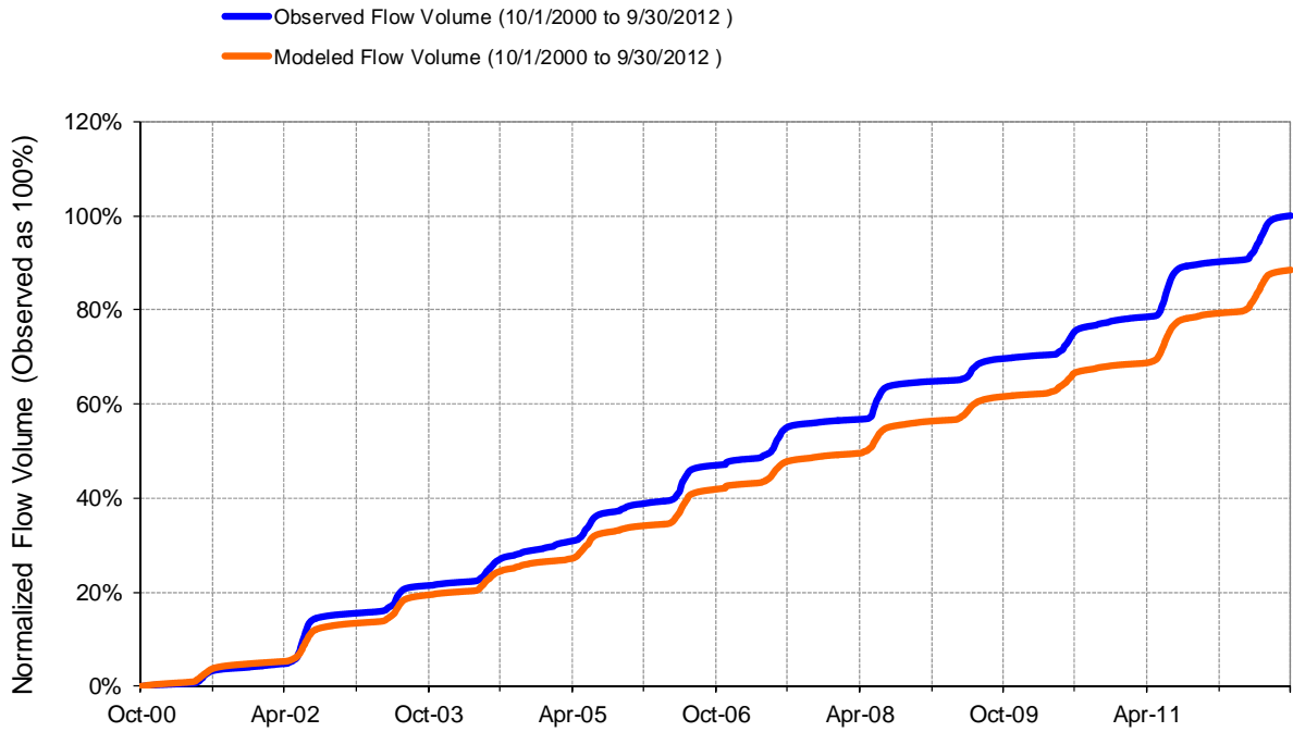
Figure G-3. Calibration Cumulative Observed and Modeled Flow Volume, USGS 12355000 Flathead River at Flathead, BC
