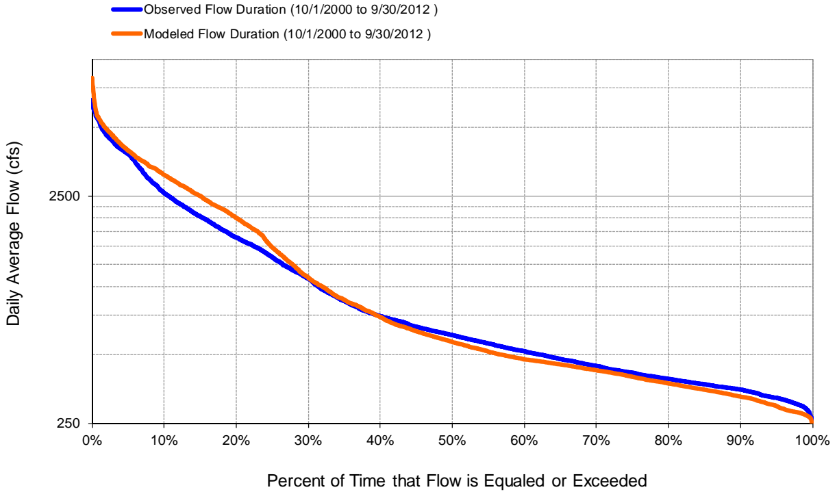
Figure G-36. Calibration Observed and Modeled Flow-Duration, USGS 12370000 Swan River near Bigfork, MT
