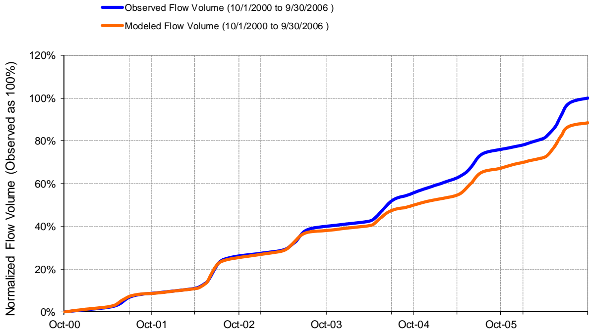
Figure G-28. Calibration Cumulative Observed and Modeled Flow Volume, USGS 12366000 Whitefish River near Kalispell, MT
