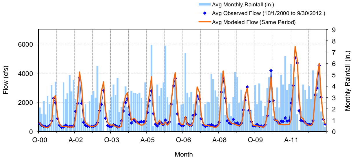
Figure G-37. Calibration Time Series of Observed and Modeled Monthly Flows and Monthly Rainfall, USGS 12370000 Swan River near Bigfork, MT
