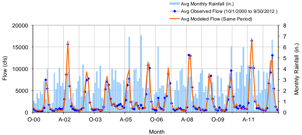
Figure G-12. Calibration Time Series of Observed and Modeled Monthly Flows and Monthly Rainfall, USGS 12358500 M F Flathead River near West Glacier, MT
