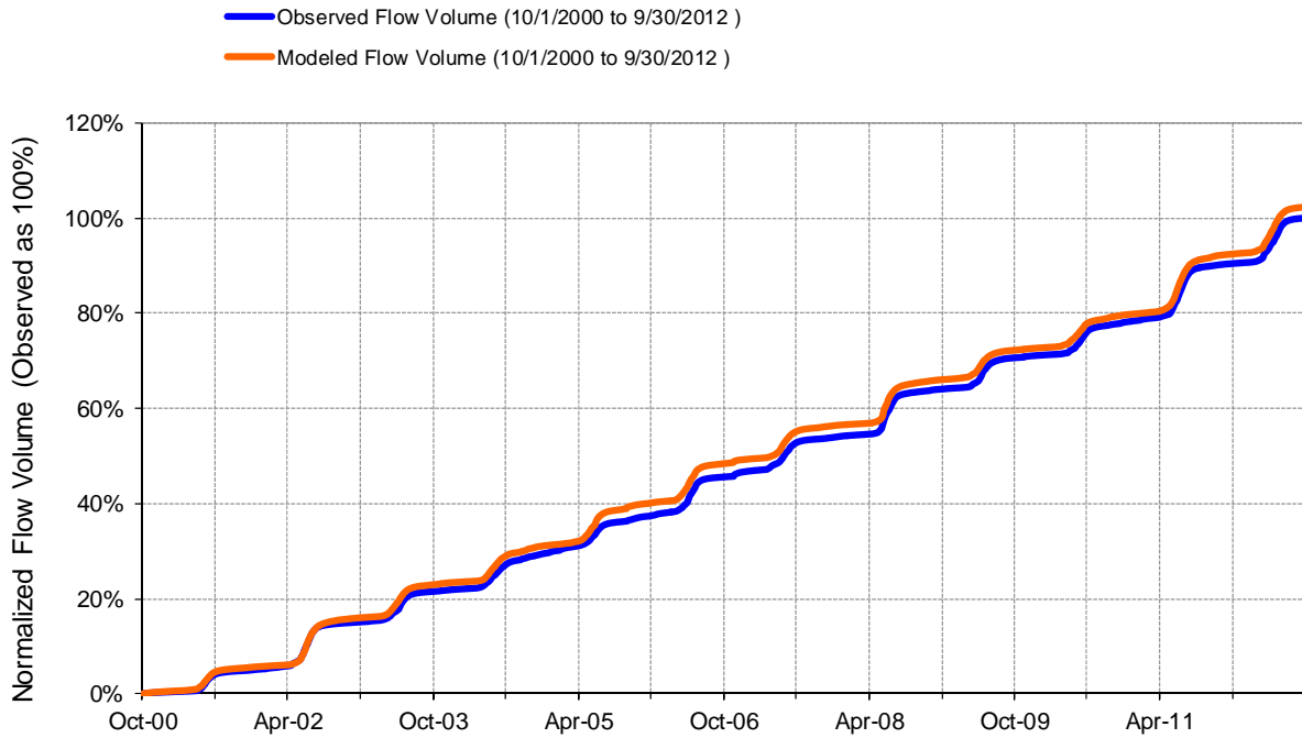
Figure G-13. Calibration Cumulative Observed and Modeled Flow Volume, USGS 12358500 M F Flathead River near West Glacier, MT
