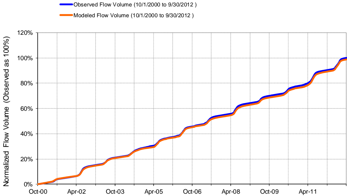
Figure G-18. Calibration Cumulative Observed and Modeled Flow Volume, USGS 12363000 Flathead River at Columbia Falls, MT
