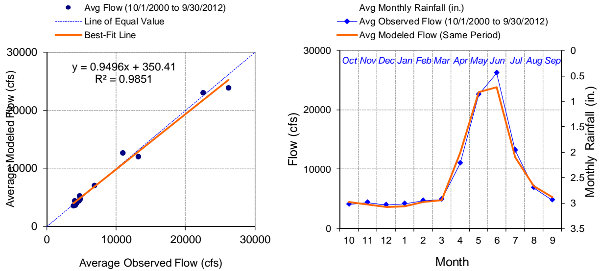
Figure G-20. Calibration Observed and Modeled Monthly Average Flow with Monthly Rainfall, USGS 12363000 Flathead River at Columbia Falls, MT
