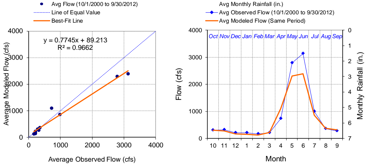
Figure G-5. Calibration Observed and Modeled Monthly Average Flow with Monthly Rainfall, USGS 12355000 Flathead River at Flathead, BC
