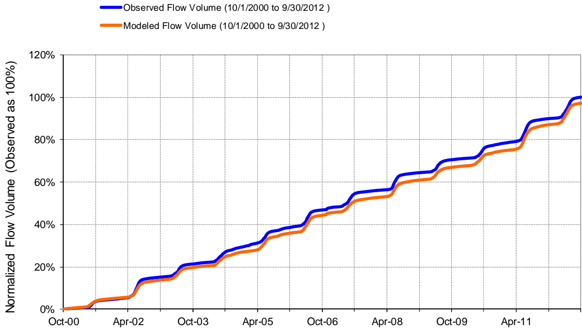
Figure G-8. Calibration Cumulative Observed and Modeled Flow Volume, USGS 12355500 N F Flathead River nr Columbia Falls, MT
