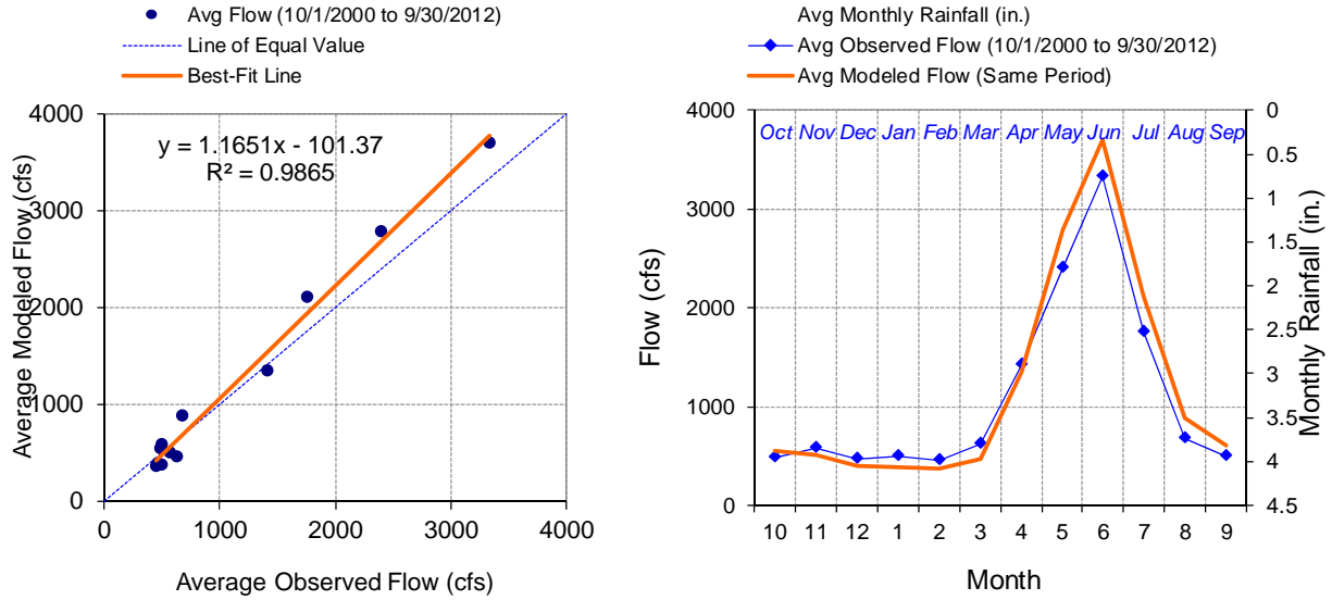
Figure G-40. Calibration Observed and Modeled Monthly Average Flow with Monthly Rainfall, USGS 12370000 Swan River near Bigfork, MT
