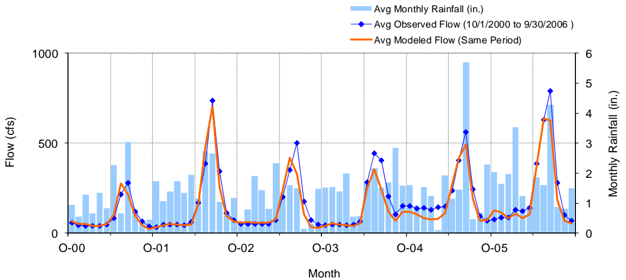
Figure G-27. Calibration Time Series of Observed and Modeled Monthly Flows and Monthly Rainfall, USGS 12366000 Whitefish River near Kalispell, MT
