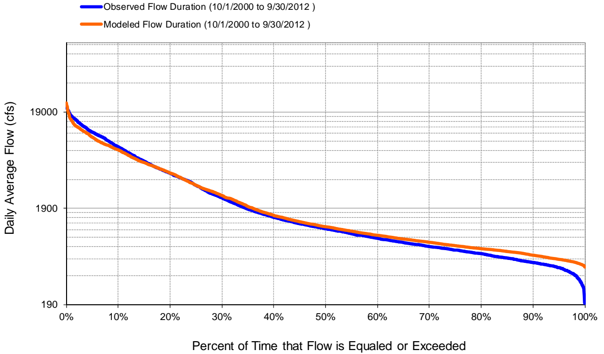
Figure G-6. Calibration Observed and Modeled Flow-Duration, USGS 12355500 N F Flathead River nr Columbia Falls, MT
